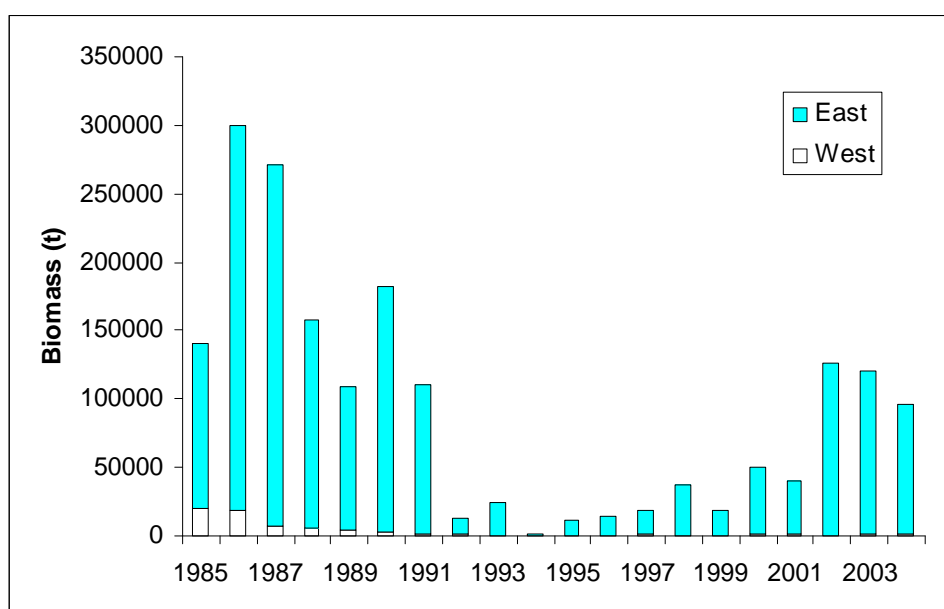
Figure 1.4.7.2 S. marinus ( \geq 17 cm). Survey biomass indices for East and West Greenland, 1985–2004.
