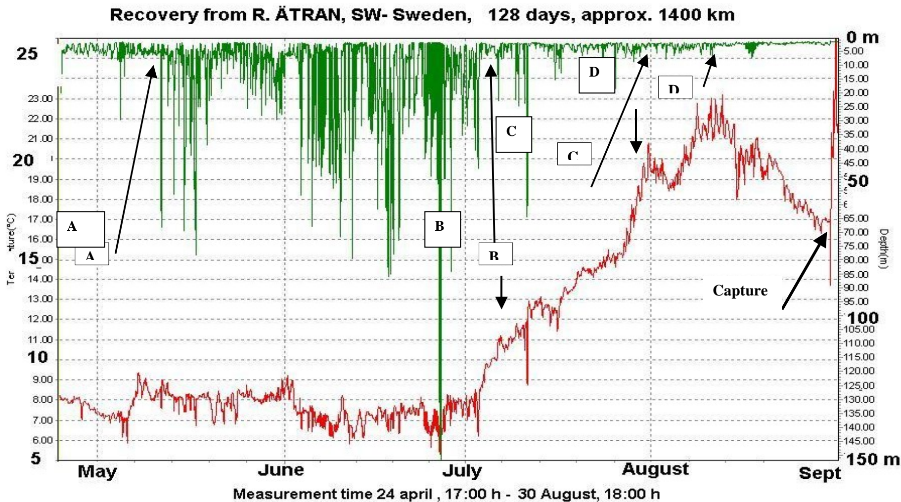
Figure 2.3.5.4.1 Data records of a salmon recovered in R. Ätran, Sweden. Depth above and temperature track below. To the left of A) post-release period , and probable periods of B) feeding and migration activity, C) Coastal migration (rising temperature), D) Estuarine dwelling and migration followed by in-river dwelling when the diving activity ceases.
