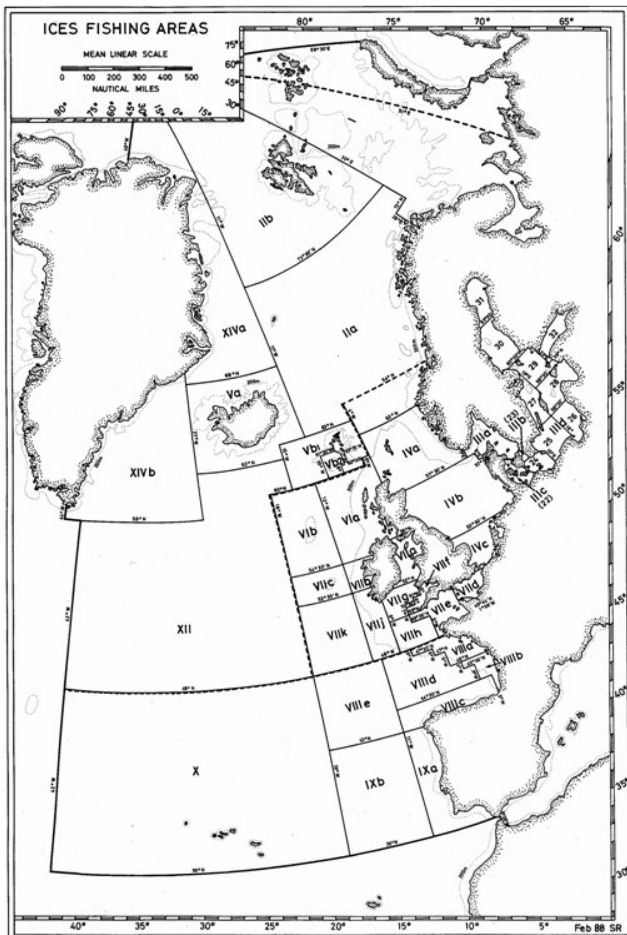
Figure 3.11.1.1 ICES fishing Areas.
