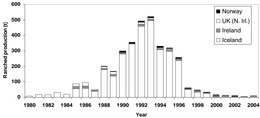
Figure 2.2.2. Production of ranched salmon (tonnes round fresh weight) as harvested at ranching facilities in the North Atlantic, 1980-2004.
