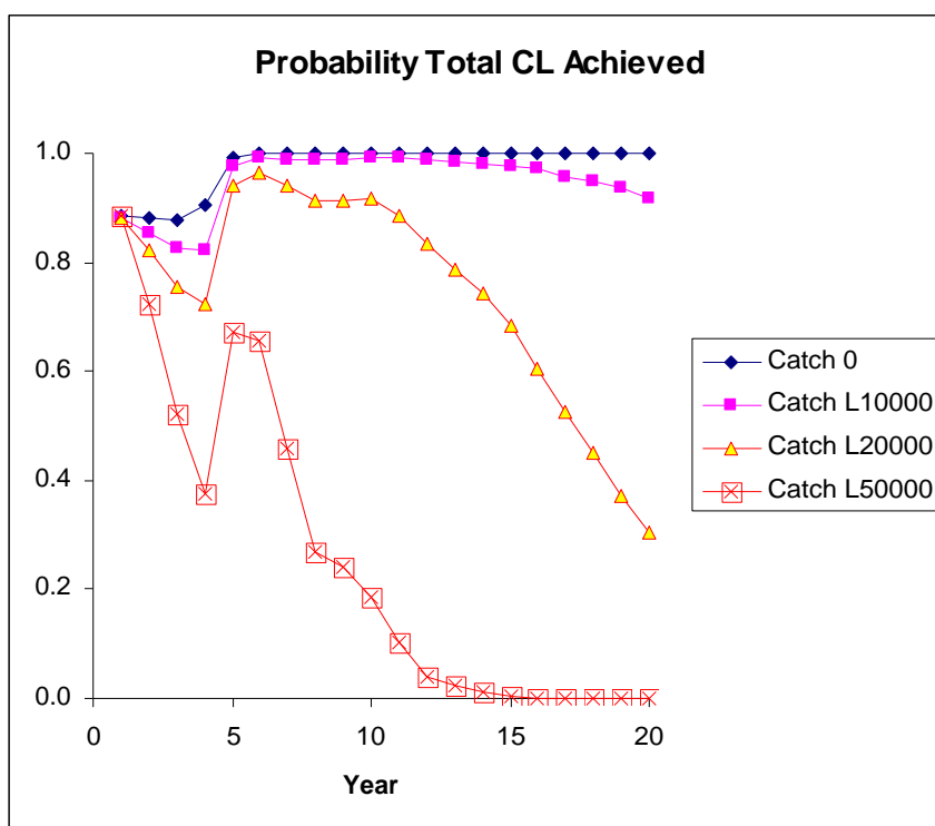
Figure 2.3.5.3.1 Probability that the total CL is achieved in the district each year under four levels of catch.
