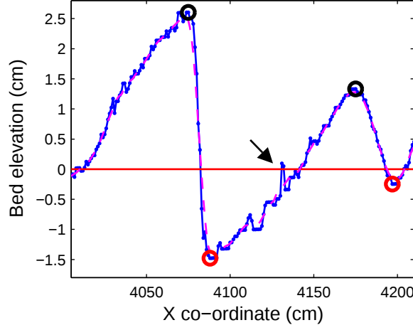
Figure 6: A filter is needed to prevent that a small disturbance that crosses the zero line is considered to be a bedform. The dashed line indicates the filter. Part of a BEP of experiment T5 of Blom et al. (2003) is shown.
