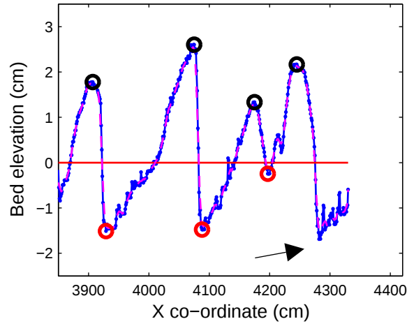
Figure 10: A trough is located at the boundary of the BEP. This trough is not recognized as such, as it is not surrounded by two crossings. Part of a BEP of experiment T5 of Blom et al. (2003) is shown.
