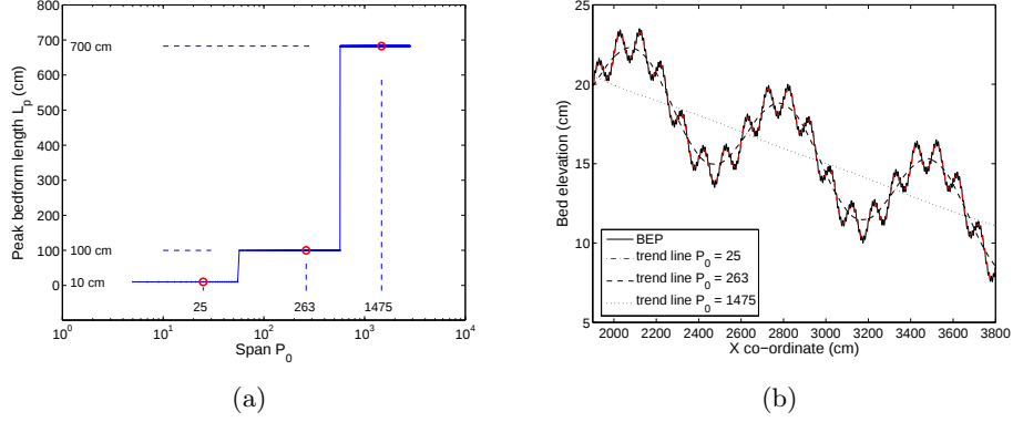
Figure 30: Illustration of the trend lines corresponding to dominant bedform lengths for example 2. a) Peak bedform length against the trend line span. The horizontal parts (sills) indicate the dominant bedform lengths. b) Original BEP together with the trend lines (dashed) determined with a span of P_0 = 25 , 263 and 1475.
