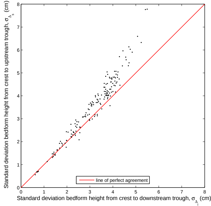
Figure 21: Comparison between \sigma_{\Delta_s} , the standard deviation of bedform height determined as the vertical distance from crest to upstream trough, and \sigma_{\Delta_l} , the standard deviation of bedform height determined as the vertical distance from crest to downstream trough.
