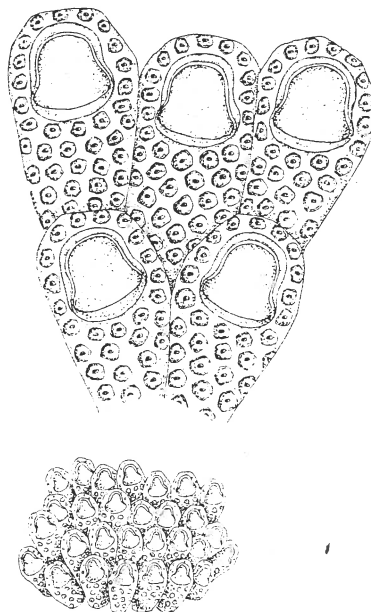
Fig. 1. Cryptosula pallasiana
