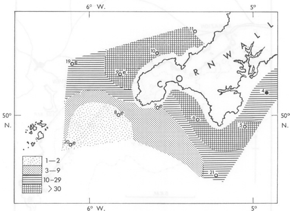
Fig. 6. Distribution of young fish (3-20 mm length) off West Cornwall, 4-5 April. Samples taken with modified Gulf III high-speed sampler, fitted with 40 m.p.i. net. Results are expressed as numbers per haul, corrected to a flowmeter reading corresponding to approximately 40 cubic metres of water filtered. All samples except one (solid black circle) were taken in daylight. The letter 'e' shows the occurrence of north-western type of plankton, a predominance of the arrow-worm Sagitta elegans and/or the presence of larvae of the starfish Luidia sarsi .
