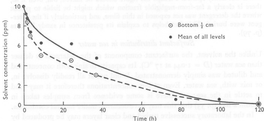
Fig. 2. Rate of loss of solvent fraction of BP 1002 from large volume of 10 ppm solution in sea water in open container.
