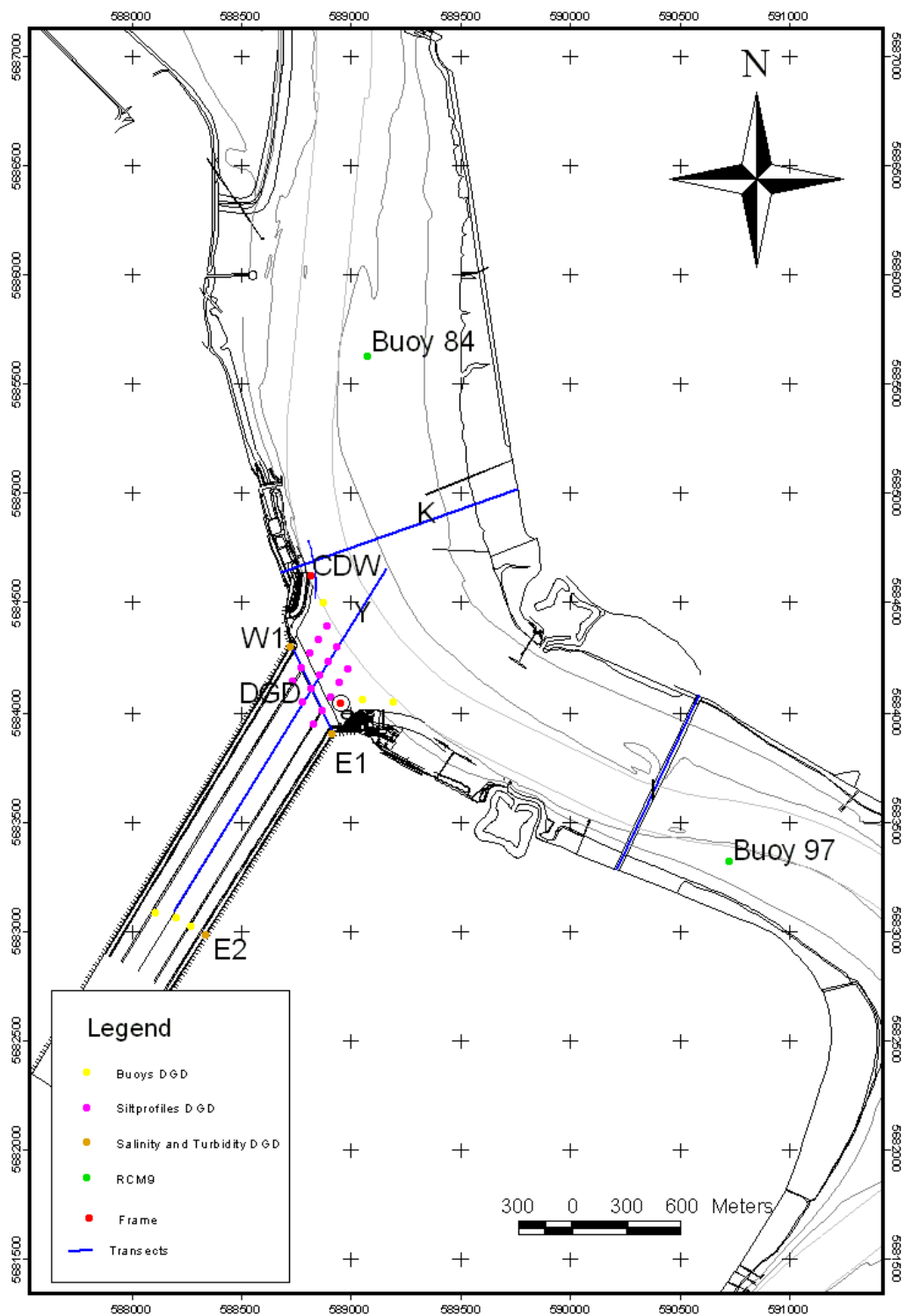
Annex Figure A-2: Overview of the measurement locations at Deurganckdok during previous campaigns
