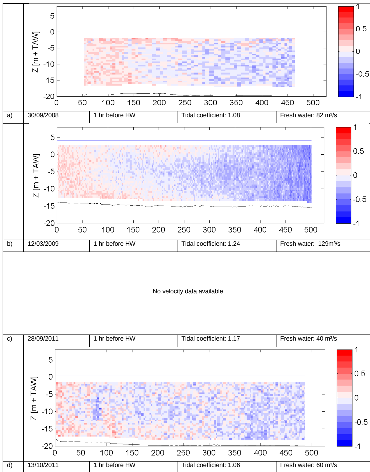
Figure 5-6: Perpendicular current velocity at 1hr before high water
