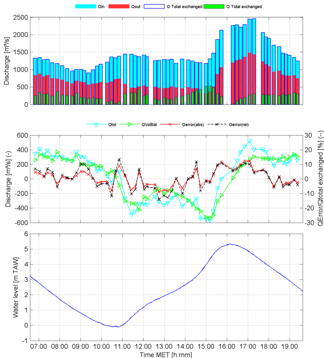
Figure 5-8: The water discharge at the entrance of Deurganckdok over a tidal curve on 13/10/2011. Top: Total incoming ( Q_{in} ) and outgoing ( Q_{out} ) discharge including the total water en tidal exchange; Central: Measured residual discharge ( Q_{tot} ) versus theoretical residual discharge ( Q_{VolBal} ) and correction offset ( Q_{error} ) including relative error; Below: tidal curve.
