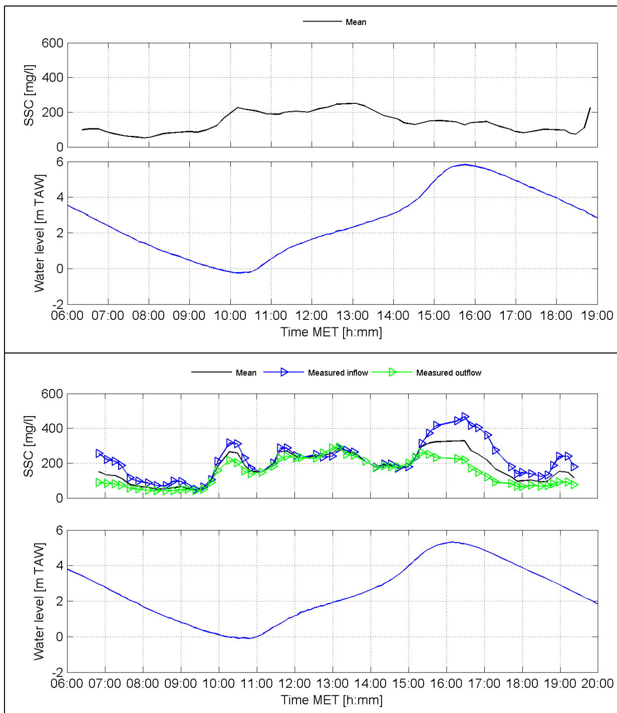
Figure 5-1: Incoming, outgoing and averaged SSC over a complete tidal cycle on 28/09/2011 (top) and 13/10/2011 (below)
