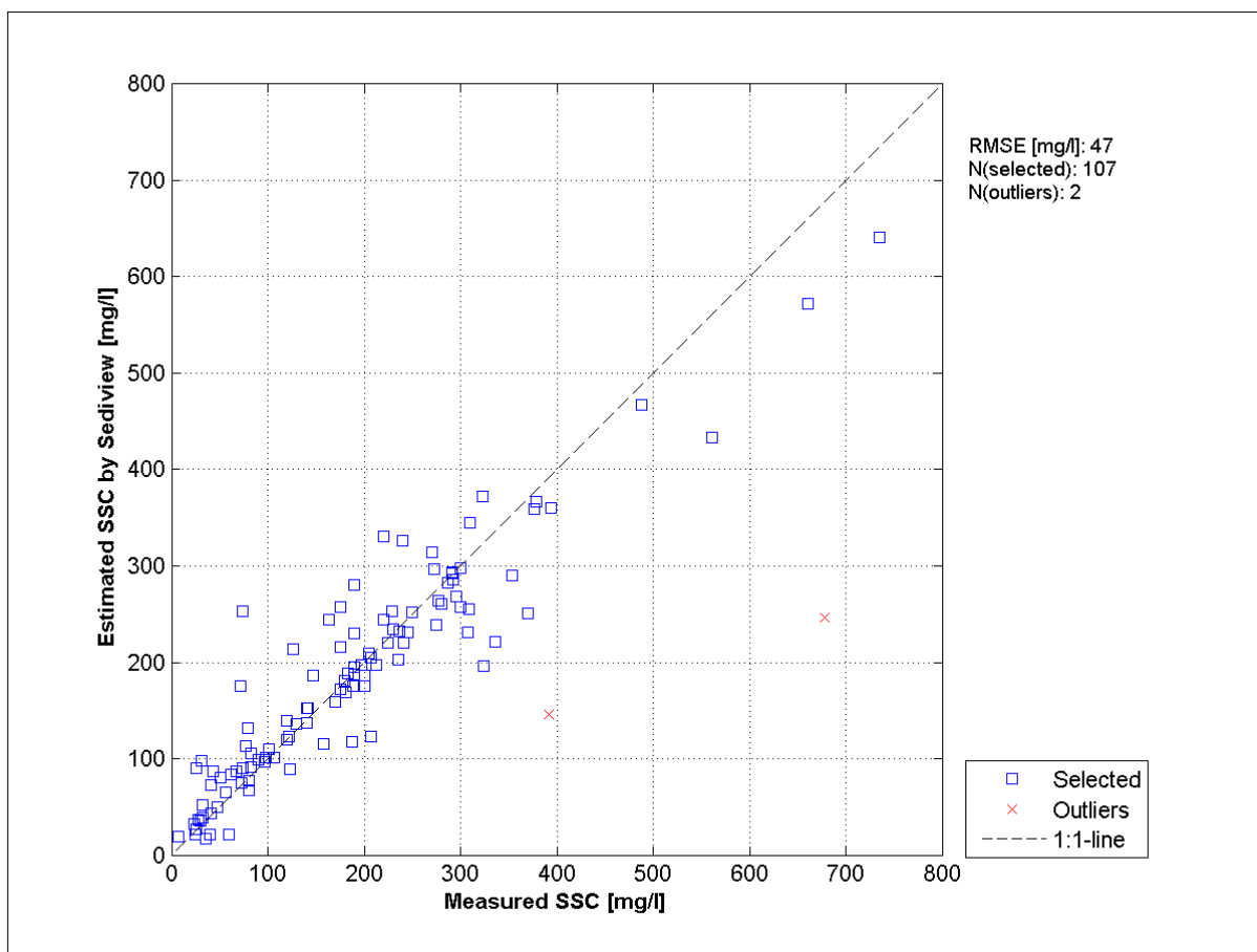
Annex Figure E-2: Calibration in Sediview for 13/10/2011 data
