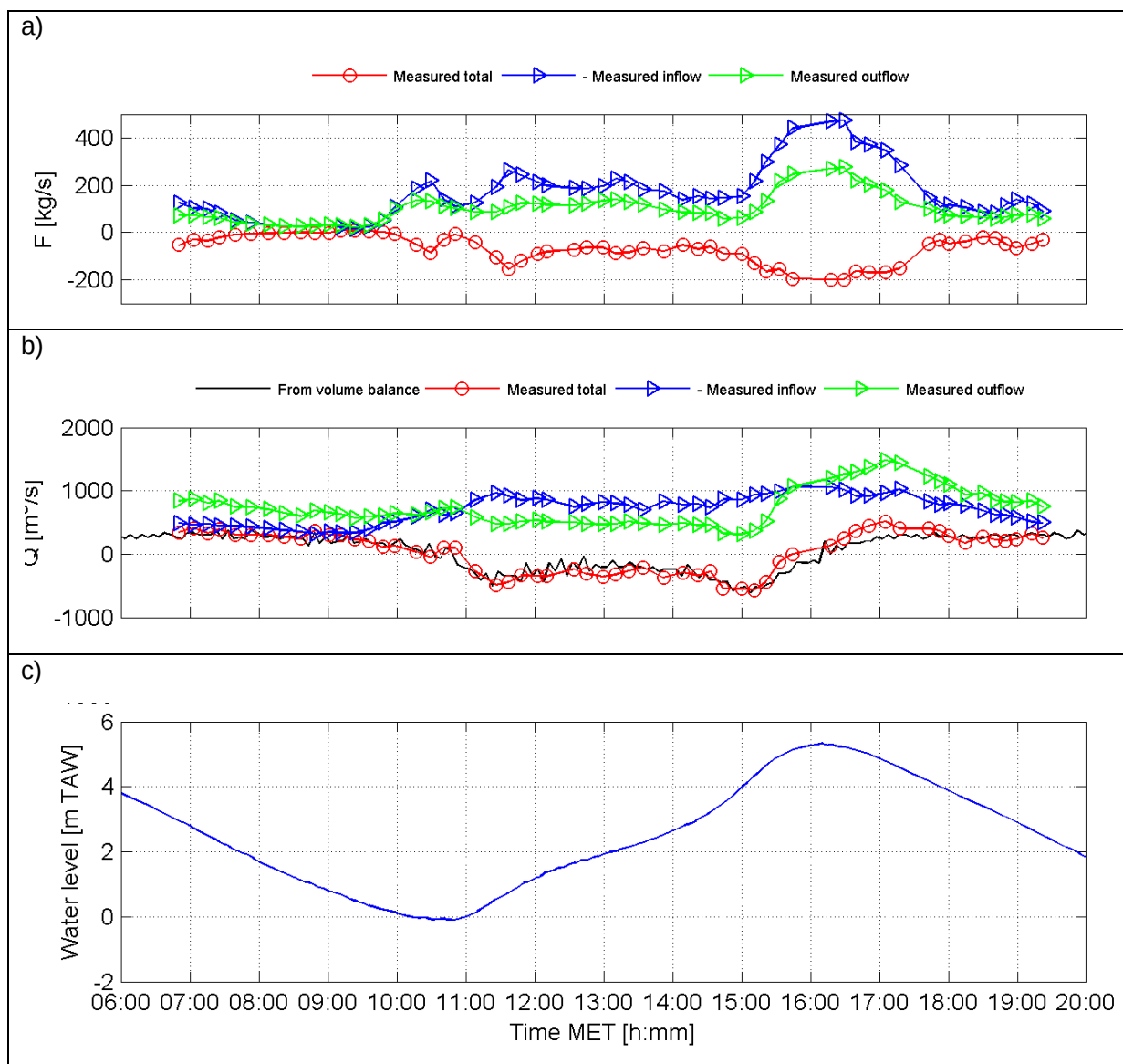
Figure 5-2 Total in/out/net flux a) and in/out/net discharge b) at DGD on 13/10/2011.
