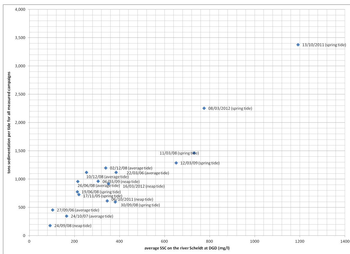
Figure 5-10 Overview of measured sediment deposition in Deurganckdock per tide by means of Sediview technique
