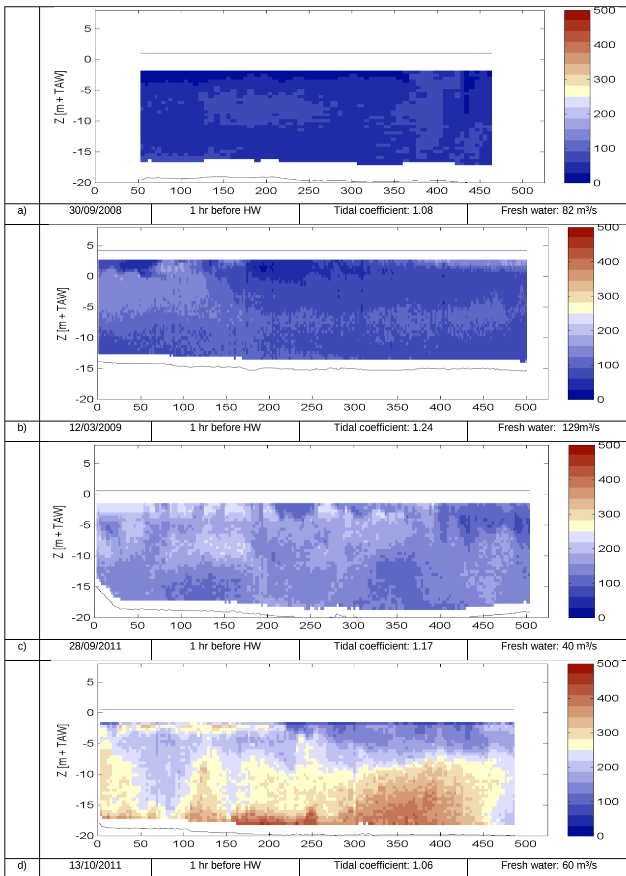
Figure 5-7: Suspended sediment concentration at 1hr before high water
