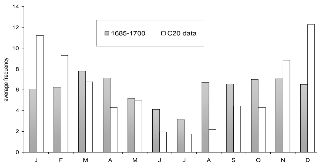
Fig. 3. Monthly mean frequencies of days with winds of Beaufort force 8 or more for the period 1685-1700 (shaded) and for the mid-twentieth century.
