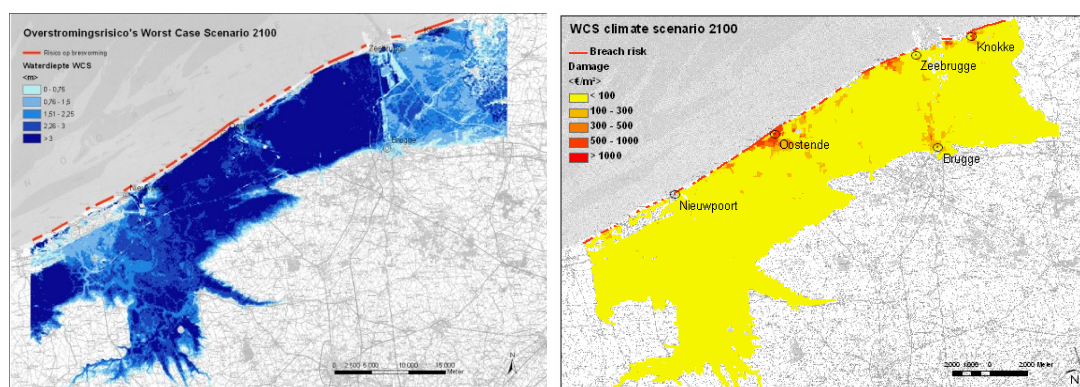
Figure 13: Results of the flood risk calculations for an extreme storm for the Worst Case 2100 scenario. Left: water depth, right: total damage.
