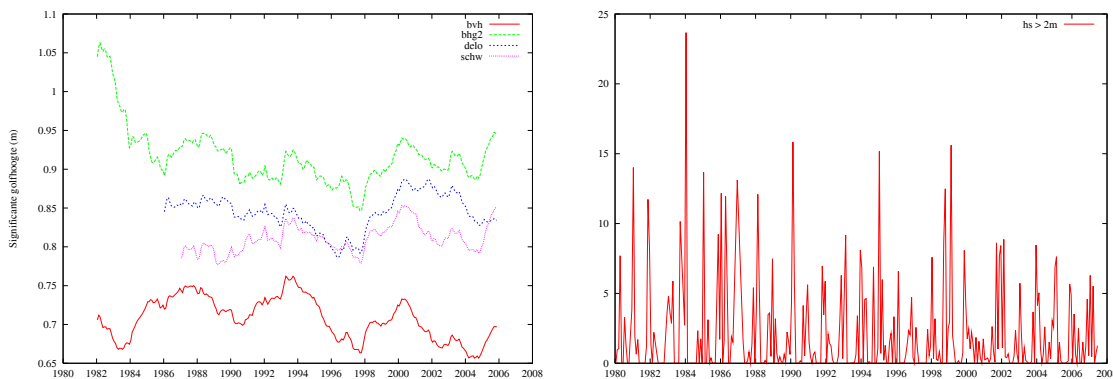
Figure 4: (a) Left: Long term trend of the monthly mean significant wave height at four measuring stations Bol van Heist (bv), Brouwershavensche Gat 2 (bhg2), Deurloo (delo) and Scheur West (schw) for the period 1980-2007. (b) Right: Percentage significant wave
