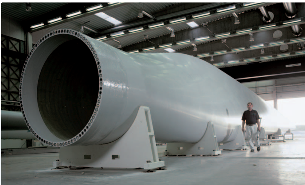
Blade factory in Nakskov, Denmark (© Vestas)
