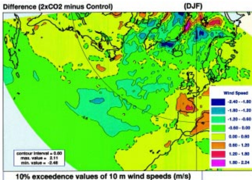
FIG. 14. Change in the intraannual 90% quantiles of wind speed as derived from a paired atmospheric circulation model run with present and doubled carbon dioxide conditions. Units: \text{m s}^{-1} . (From Beersma et al. 1997.)
