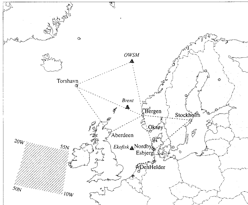
FIG. 2. Location of in situ data used in the WASA studies. Locations explicitly used in the present paper are marked by their names. Dots represent pressure gauges used for geostrophic wind calculations by Alexandersson et al. (1998). Triangles: Tide gauges for which high water level percentiles were calculated, and offshore stations and ocean weather stations. Geostrophic triangles used in the present article are marked by dotted lines; the wave chart area west of Ireland is marked by hatching.
