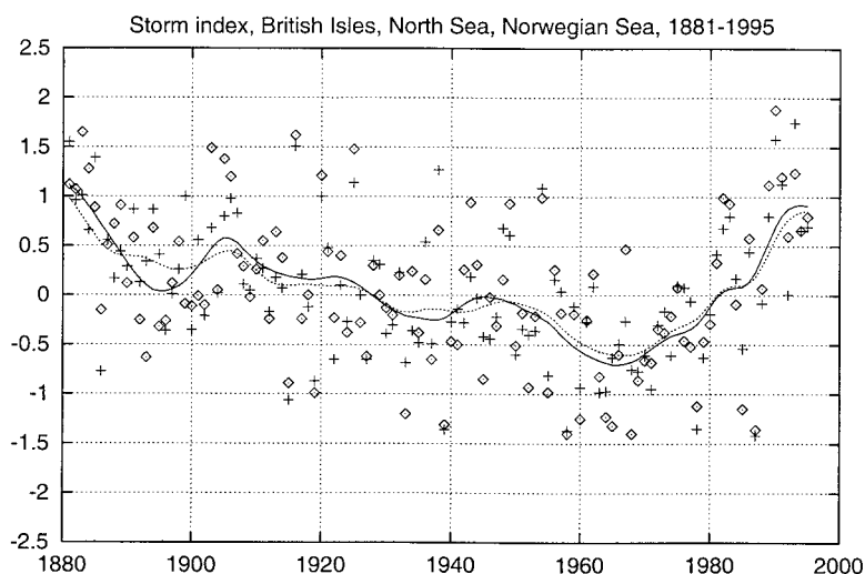
FIG. 5. Standardized annual 95% (diamonds and full line) and 99% (crosses and dotted line) quantile time series from pressure triangles in the British Isles, North Sea, and Norwegian Sea regions. The lines are obtained from the yearly data by applying a Gaussian filter with standard deviation of 3 yr. Dimensionless units. (From Alexandersson et al. 1998.)
