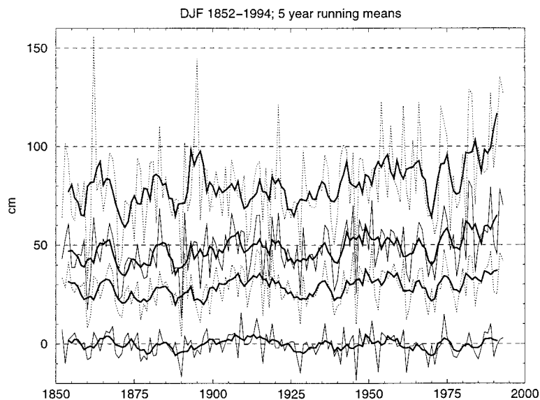
FIG. 7. Time series of the intraannual quantiles of storm-related water level variations (defined as deviation from the annual mean) at the gauges in Den Helder and Esbjerg (see triangles in Fig. 2). Units: cm.
