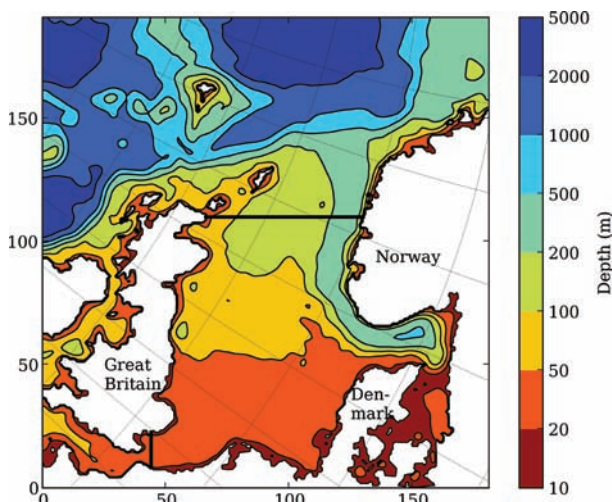
Fig. 1. Model domain with filled contours of bathymetry. Grid lines are given with 5° equidistance for longitude and 2° for latitude. The axis tick labels are grid coordinates. The thick black lines delimits a subdomain for the North Sea used for statistics presented in Section 3.
