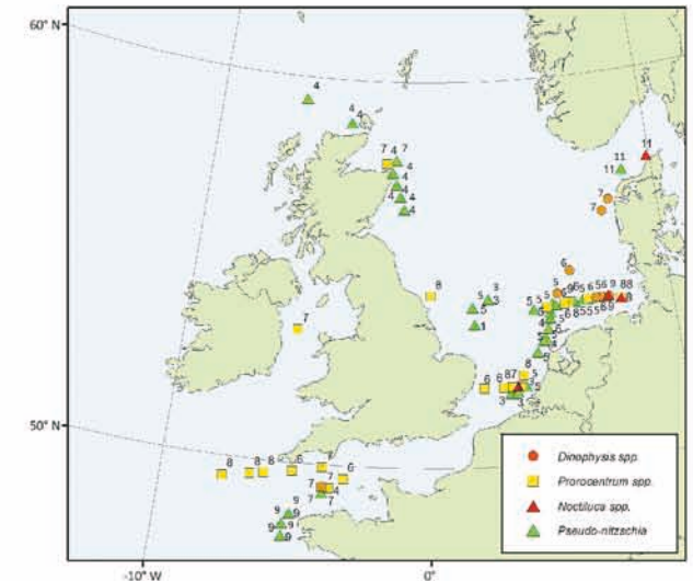
The geographical distribution of some exceptional HABs in 2009. Numbers indicate the month of the bloom.
