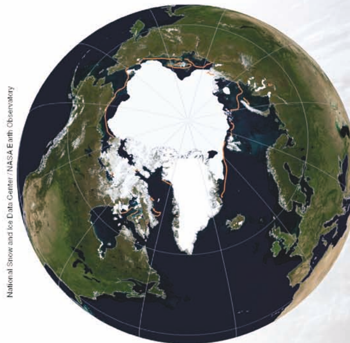
Ice extent for summer 2010
