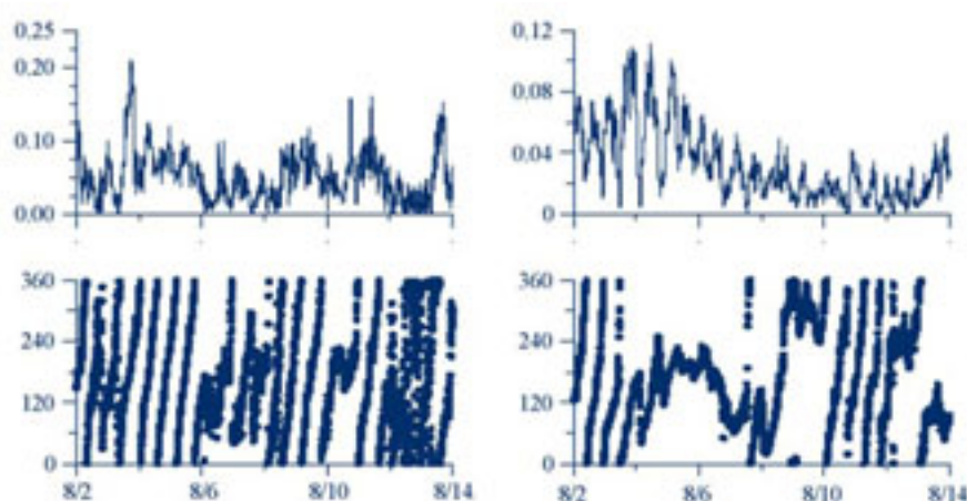
FIGURE 3: Currents as measured in location 55°28'N, 18°10'E in the period 2-14.08.96; left - depth 13 m / right - 75 m (Robakiewicz, 2004)
