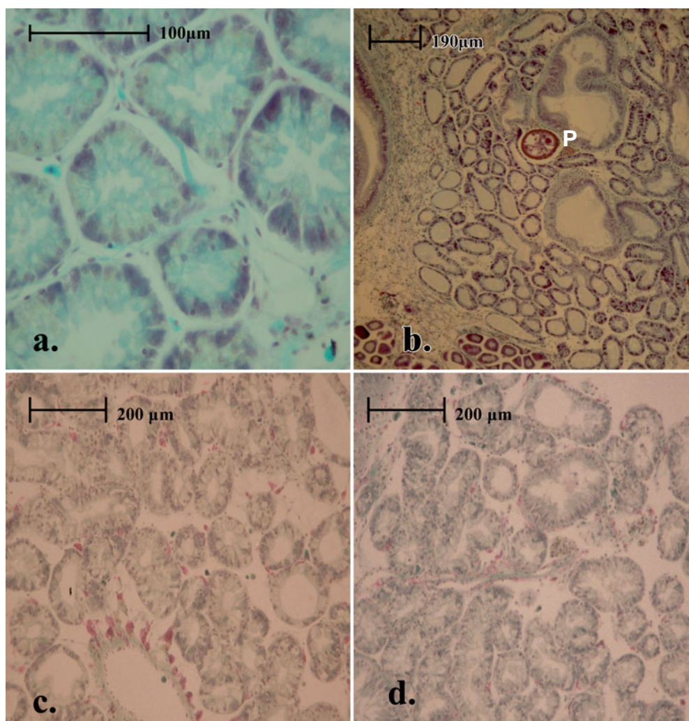
Fig. 1. Transverse sections of digestive tissue showing: (a) normal tubules at Day 0 and a normal digestive:basophil ratio; (b) typical impacted digestive cells from a separate study, illustrating thinning of tubules and the presence of a parasite (P); (c) healthy tubules and a normal digestive:basophil ratio at Day 60 in the control treatment, indicating no impact; and (d) healthy tubules and a normal digestive:basophil ratio at Day 60 in the pH 6.5 treatment, indicating no impact
