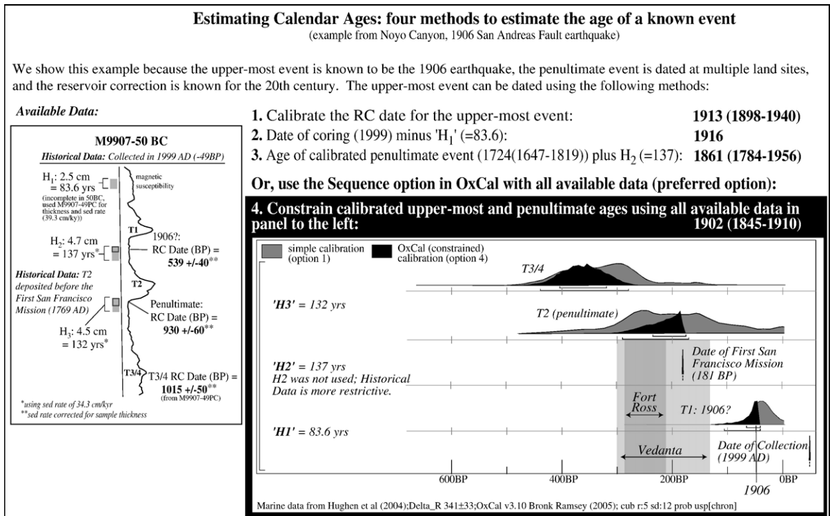
Fig. 4. OxCal methods test using the well constrained 1906 earthquake and associated paleoseismic data onshore and offshore. The left panel shows the hemipelagic (H) data determined from visual observation, physical property data mineralogy and x-radiography. H data is then input to OxCal and with raw 14 C ages are converted to time via sedimentation rate curves developed for each site. Right panel shows four ways to calculate the age of the 1906 earthquake, with the preferred method being the use of underlying and overlying hemipelagic intervals, historical data (no written record of an earthquake between the date of the first San Francisco Mission built in 1769 and 1838), and 14 C ages together. This method yields 1902 (1845–1910) for the 1906 event. The Fort Ross and Vedanta mean age and range for the penultimate event is shown, along with the OxCal solution for that event, calculated using the preferred method. The turbidite result 1660–1769 (~1760 peak) for the penultimate event is in good agreement with NSAF paleoseismic sites on land: Fort Ross=1710 (1610–1810), Vedanta=1711 (1695–1720) [28,32].
