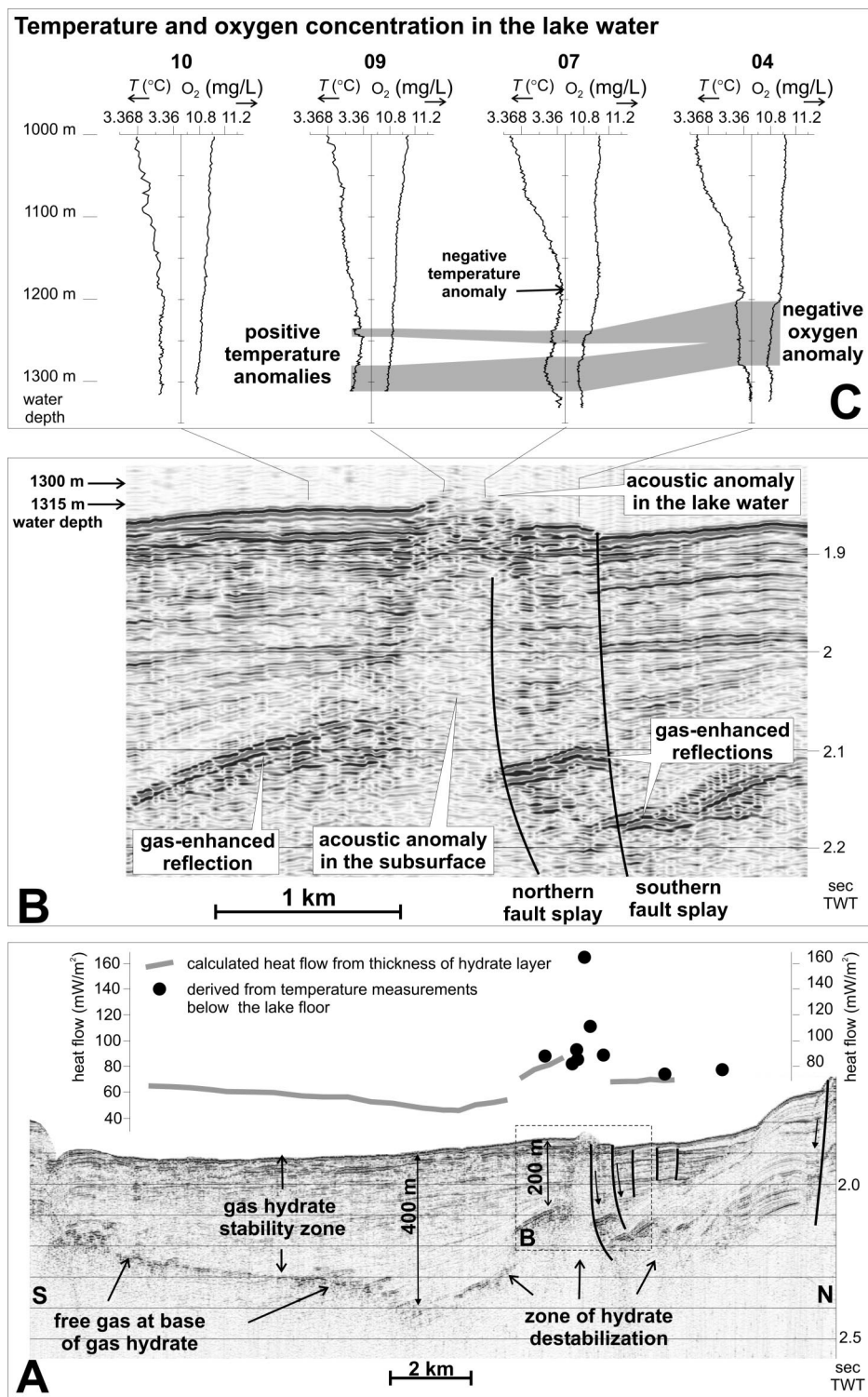
Figure 4. A: Seismic cross section showing localization of Malenki seep in its structural setting. Measured and calculated heat flow values are plotted along same profile. B: Detail of seismic section showing seismic chimney from crest of elevated base of gas-hydrate layer to lake floor at Malenki seep. Also shown is acoustic anomaly in near-bottom lake water. C: Near-bottom measurements of temperature and oxygen concentration indicate buoyant methane plume northwest of Malenki seep.
