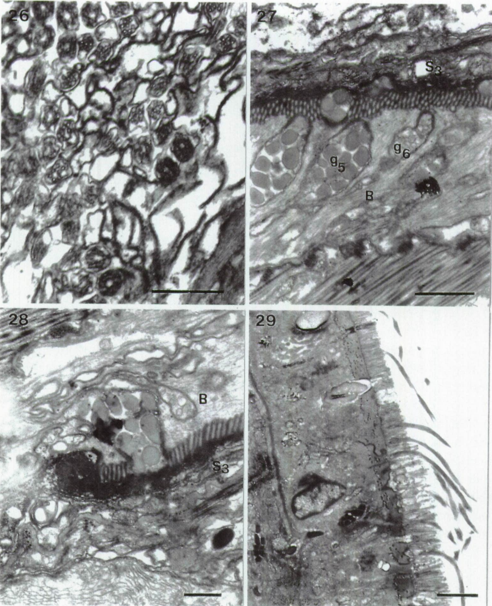
Figs 26-28. Gallorhynchus mediterraneus .
