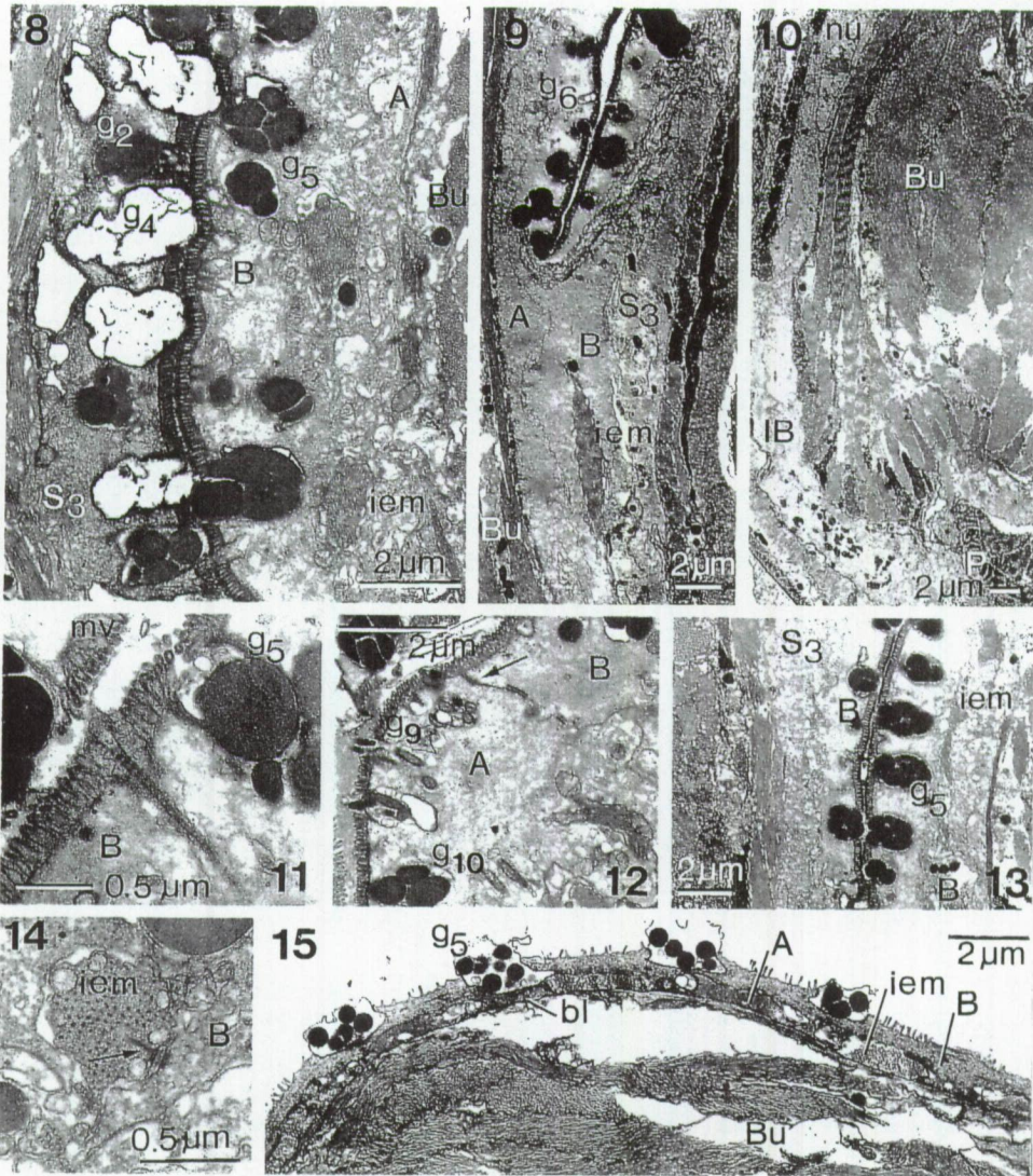
Figs. 8-14. Cystiplex axi .
