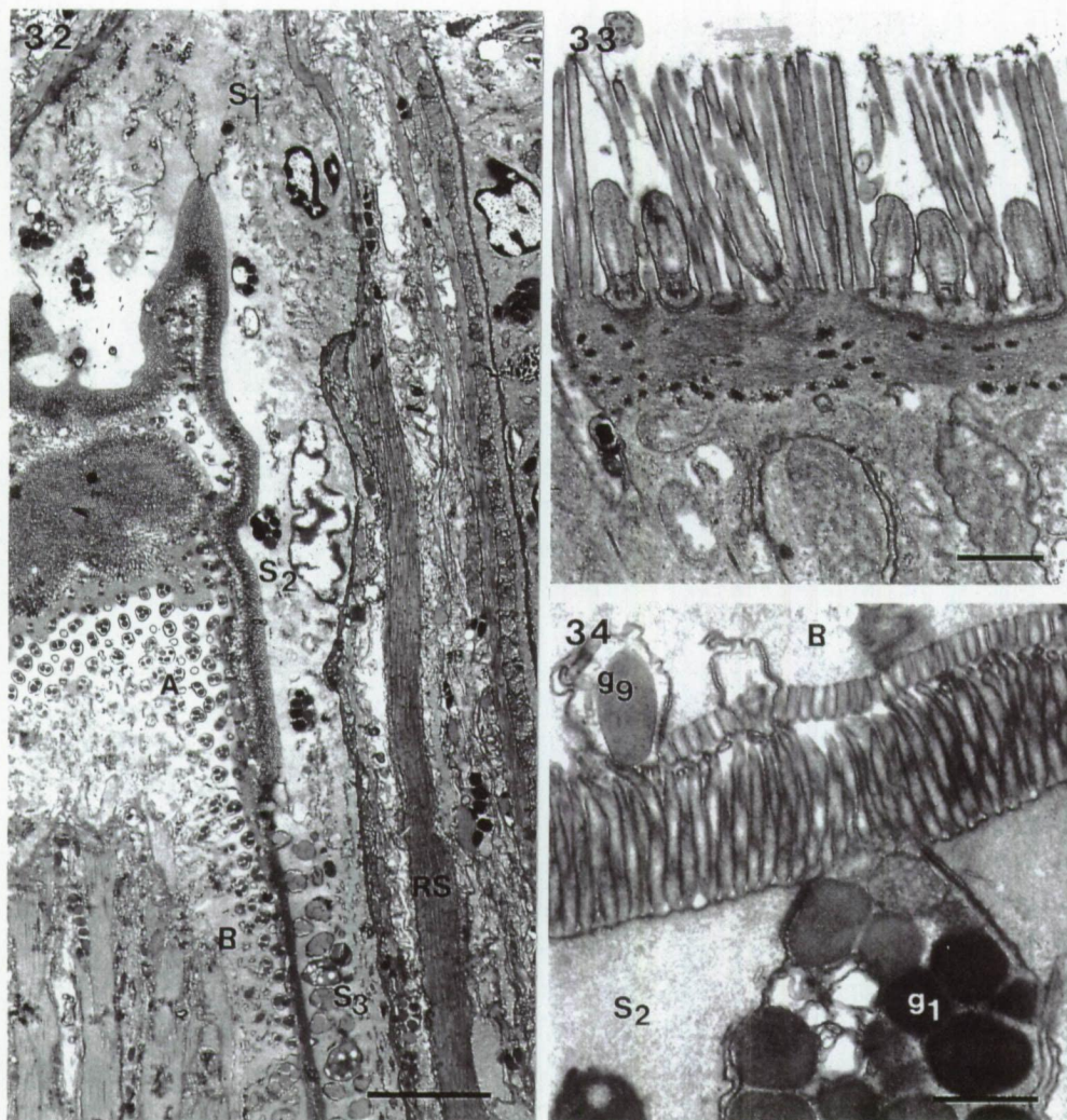
Figs 32-34. Marirhynchus longasaeta .
