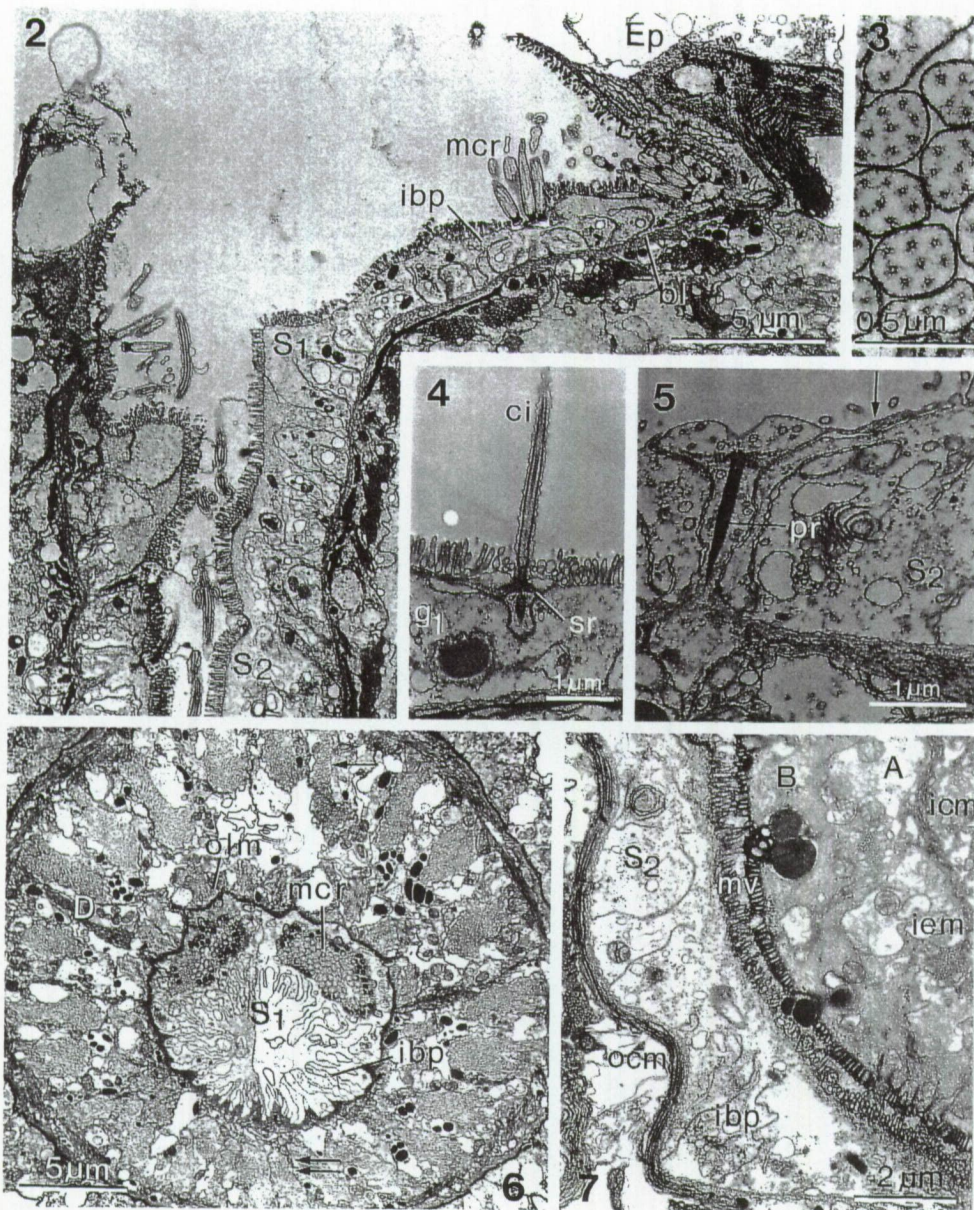
Figs. 2-7. Cystiplex axi
