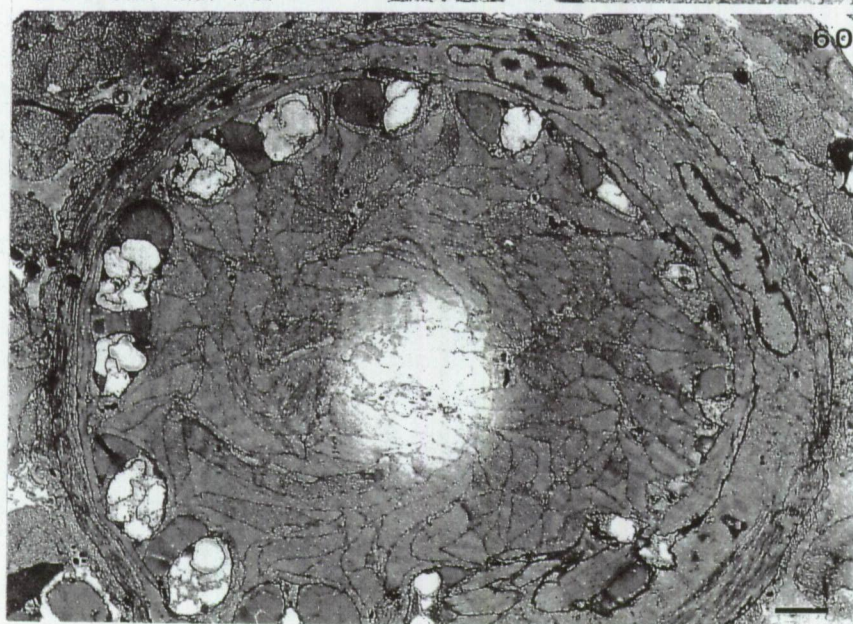
Figs. 59-60. Ptyalorhynchus coecus .
