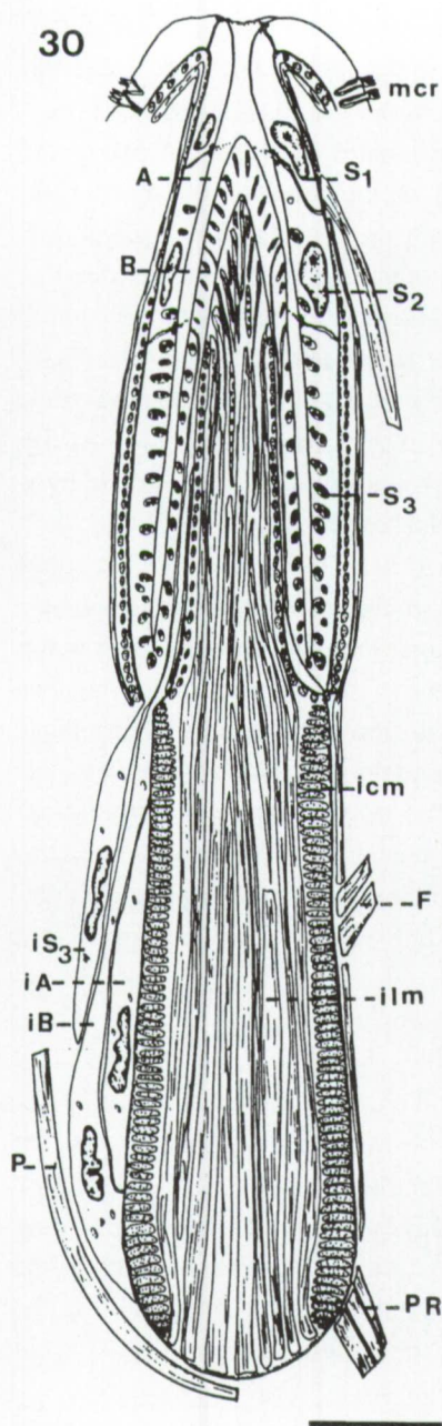
Figs 30-31. Marirhynchus longasaeta .
