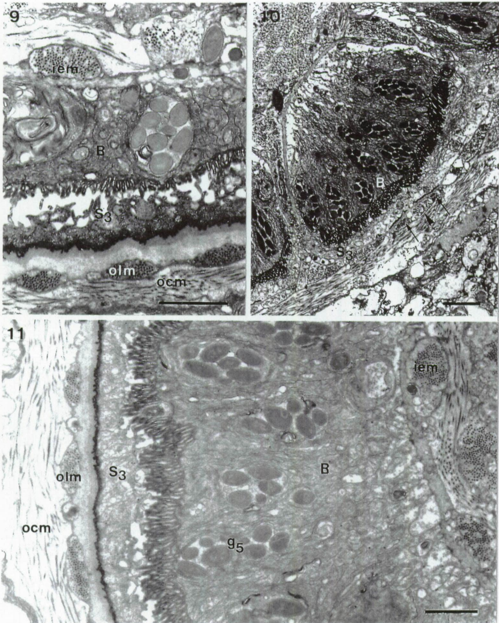
Figs 9-11. Danorhynchus gosoensis .
