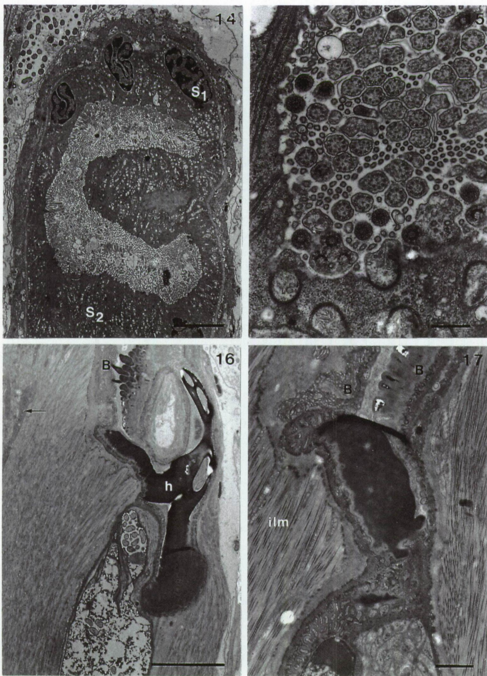
Figs 14-17. Paragnathorhynchus subterraneus .
