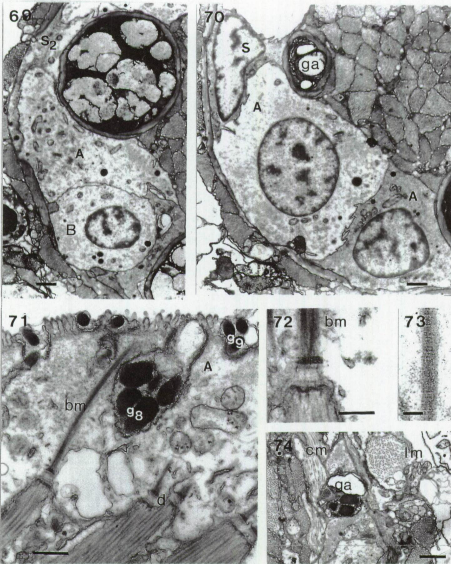
Figs 69-74. Cicerina remanei .
