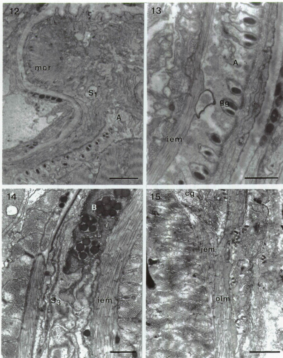
Figs 12-15. Neopolycystis tridentata .
