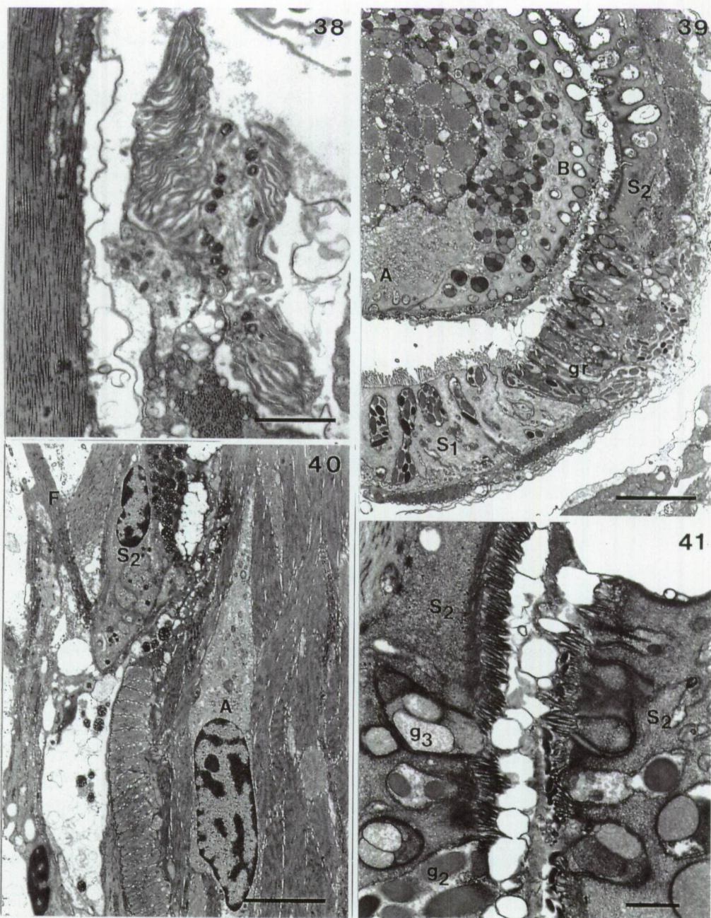
Figs 38-41. Ethmorhynchus anophthalmus .
