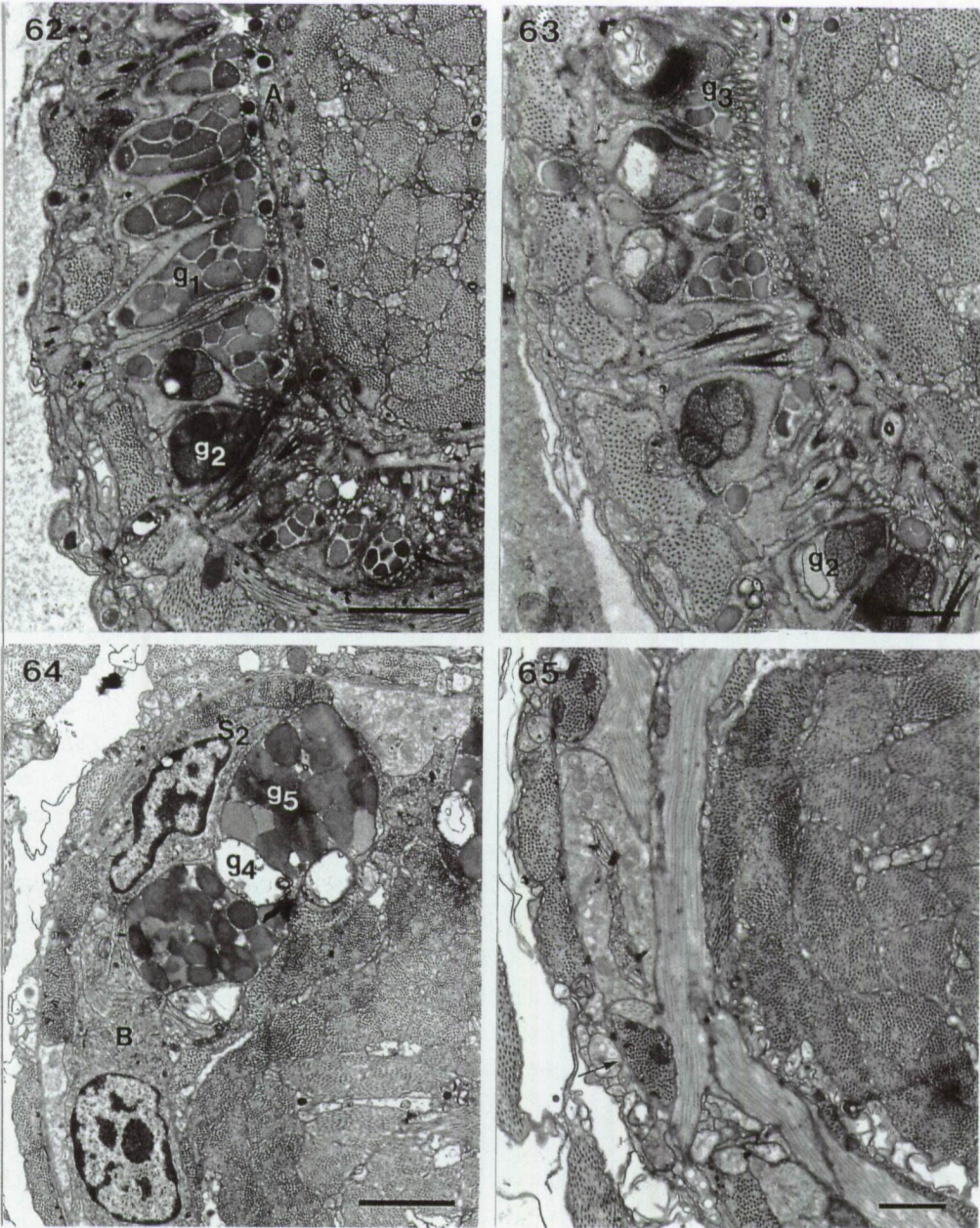
Figs. 62-65. Paracicerina deltoides .
