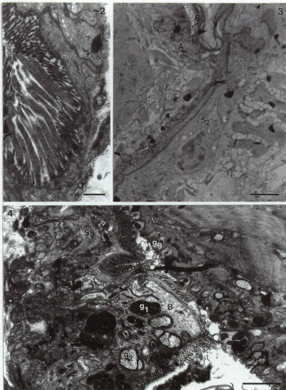
Figs. 2-4. Placorhynchus octaculeatus .
