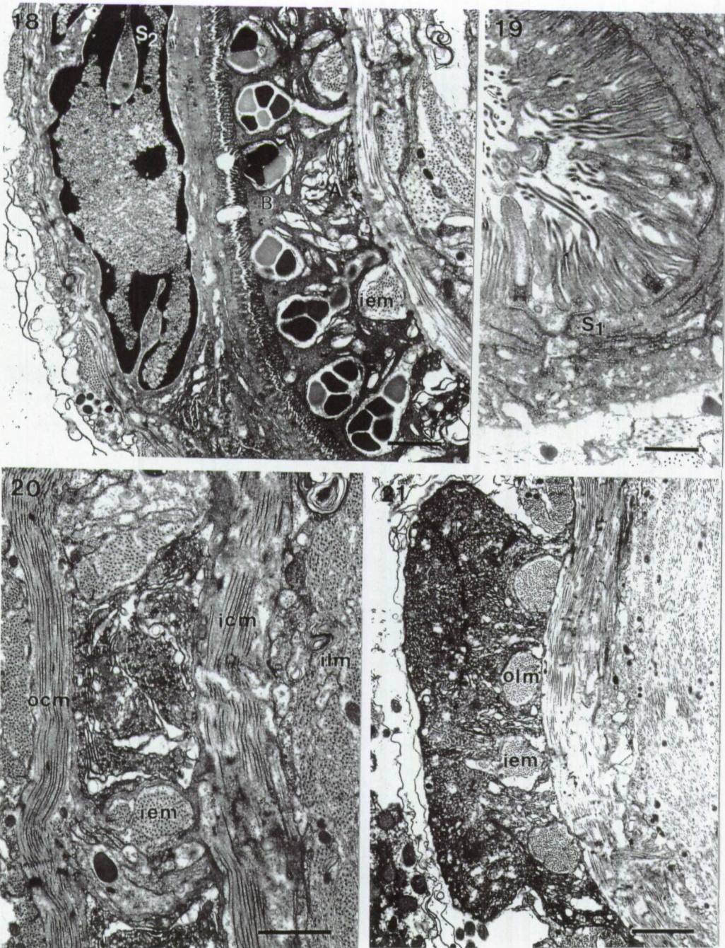
Figs 18-21. Typhlopolycystis rubra .
