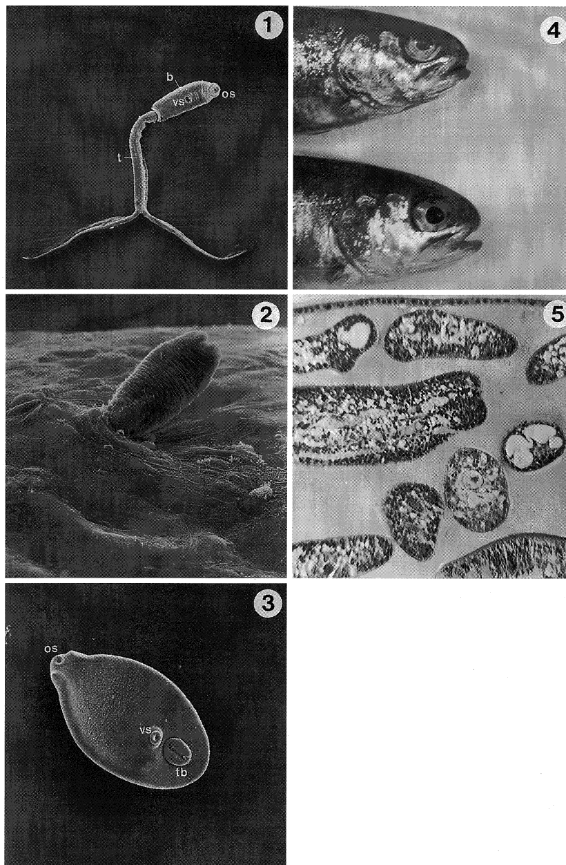
Figure 1. The cercariae of Diplostomum spathaceum obtained from Lymnaea palustris ; os=oral sucker, vs=ventral sucker, b=body, t=tail, \times 200 .
