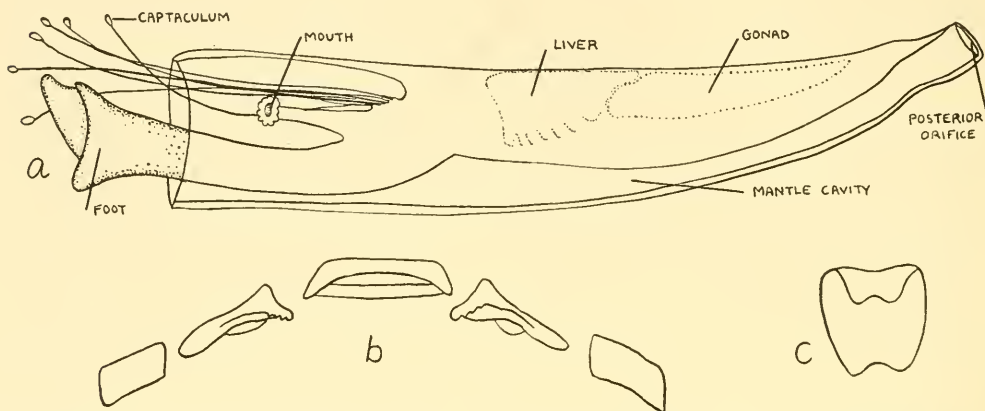
FIGURE 19. a, Diagrammatic drawing of the internal anatomy of Dentalium ; b, radular teeth of Dentalium ; c, the central tooth found in the radula of the Siphonodentaliidae .
