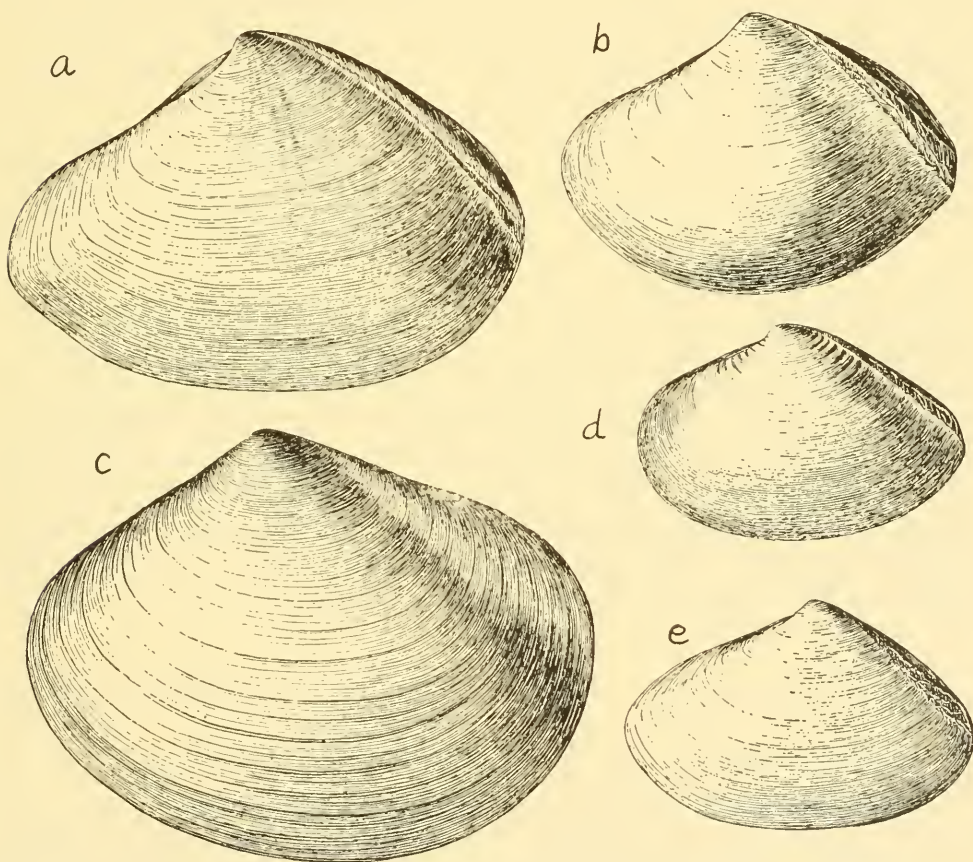
FIGURE 90. Pacific Surf Clams. a, Spisula dolabriformis Conrad, 3 inches; b, S. hemphilli Dall, 6 inches; c, Spisula catilliformis Conrad, 4 inches; d, Mactra californica Conrad, 1½ inches; e, S. planulata Conrad, 2 inches.
