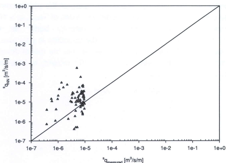
Figure 4.19 Performance of net_new for testdata of net_new with sq_{\text{measured}} < 10^{-6} \text{ m}^3/\text{s/m}
