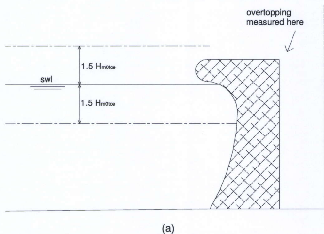
Figure 3.21 Distinction between a large (a) and a small (b) recurve wave wall
