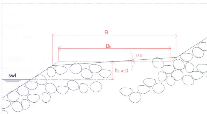
Figure 3.12 (continued) Determination of B [m], B_h [m], \tan\alpha_B [-], h_b [m]
