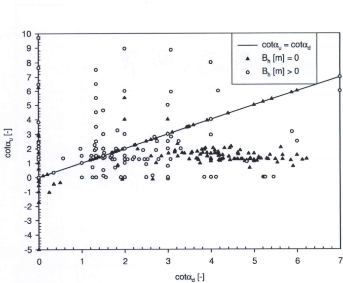
Figure 3.37 Relationship between structure slope parameters
