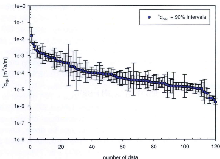
Figure 4.41 Quantifier simulation of wrongly classified data from class -1 for final criterion C
