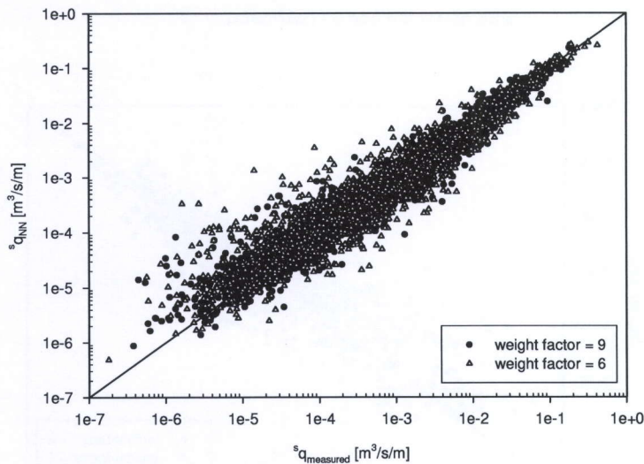
Figure 4.21 Prediction by the committee of networks for original data with weight factor = 9 and 6 (5064 data)
