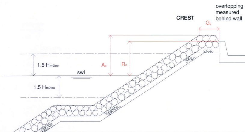
Figure 3.14 (continued-1) Determination of R_c [m], A_c [m] and G_c [m]
