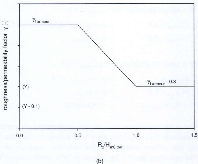
Figure 3.23 (continued) Roughness/permeability factor for (a) rough structures and (b) smooth structures
