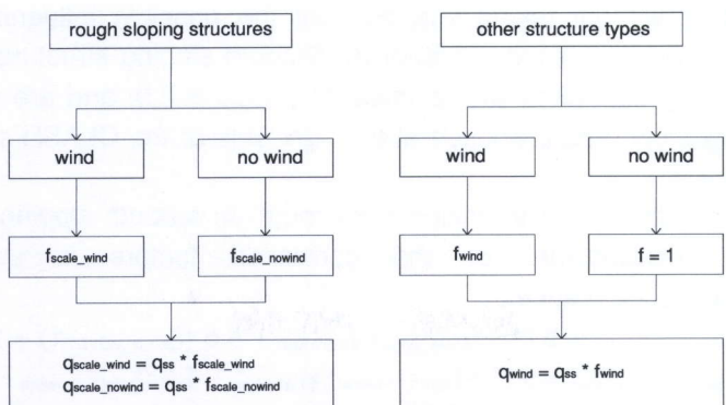
Figure 4.6 CLASH scaling map
