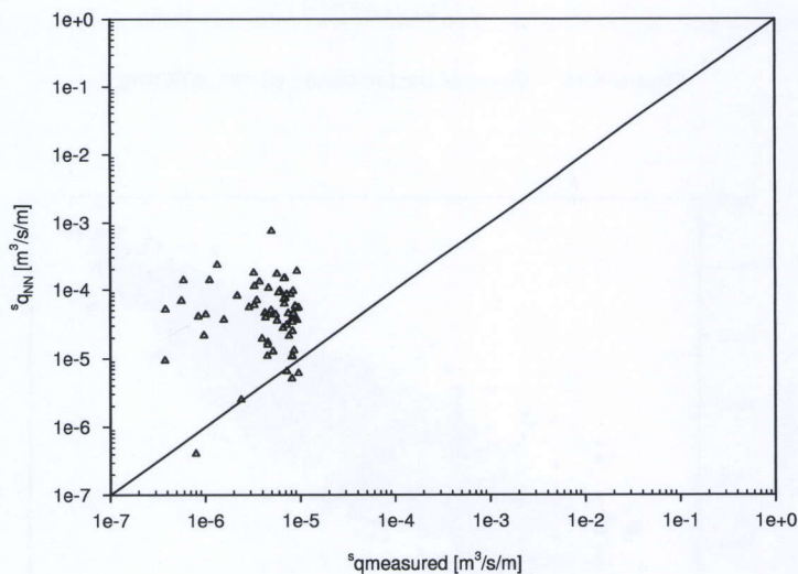
Figure 4.18 Performance of net_existing for testdata of net_new with {}^s q_{\text{measured}} < 10^{-5} \text{ m}^3/\text{s/m}
