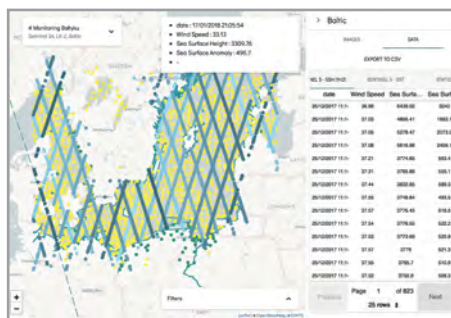
Full coverage of Baltic Sea with Sentinel-3 satellite. Sea level and temperature measurements in Maritime Spectator. Credit: Contains modified Copernicus Sentinel data [2018]
