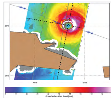
Sentinel-1 derived surface wind speed over Irma on 07/09/2017 during a category-5 hurricane, showing winds greater than 80m/s
