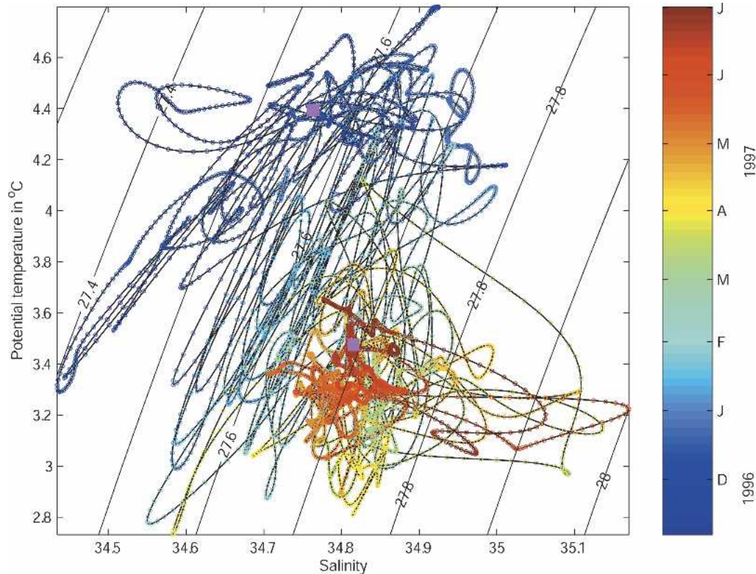
FIG. 12. A \theta - S diagram for the top instrument (108 m) at mooring K2 during the convection period. The magenta squares indicate the beginning and the end of the record. The square with the warmest temperature corresponds to the beginning of the record. The color along the curve indicates time.
