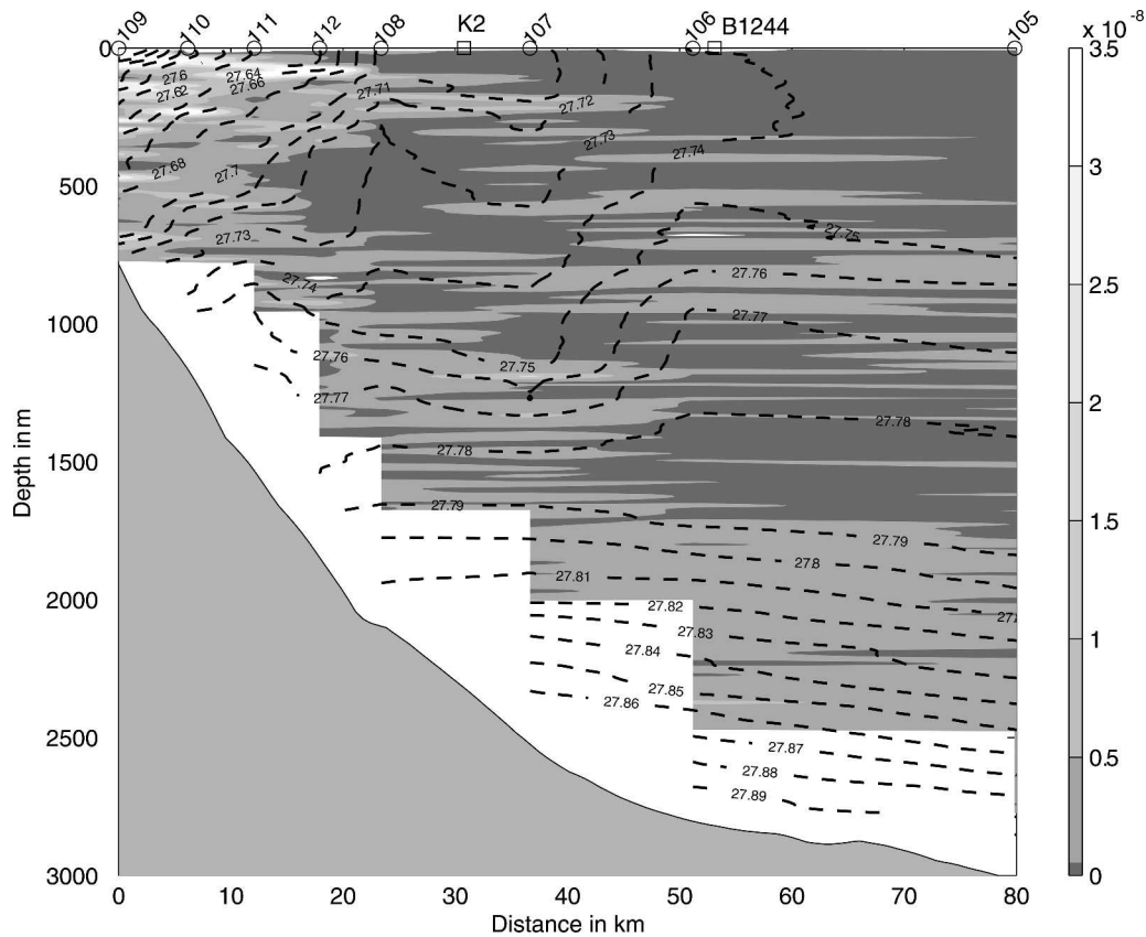
FIG. 14. Potential vorticity ( \text{s}^{-3} ) section above the Labrador slope computed from the Mar 1997 AR7W hydrographic data. Potential density \sigma_0 contours ( \text{kg m}^{-3} ) are shown with dashed lines. Note the low-PV blob in the boundary current at station 108. The squares indicate the location of mooring K2 and B1244.
