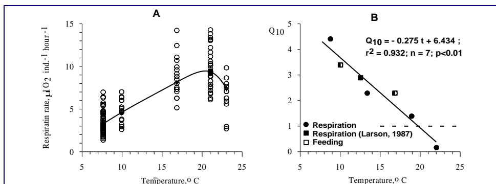
Figure 3.11. Variations in respiration rate ( \mu\text{l O}_2 \text{ ind.}^{-1} \text{ hour}^{-1} ) (A) and temperature acceleration of metabolic rate ( Q_{10} ) (B) for 1g WW Aurelia aurita depending on seawater temperature ( ^{\circ}\text{C} ). Dotted line corresponds to the maximum rate of the metabolism ( Q_{10} = 1 )
