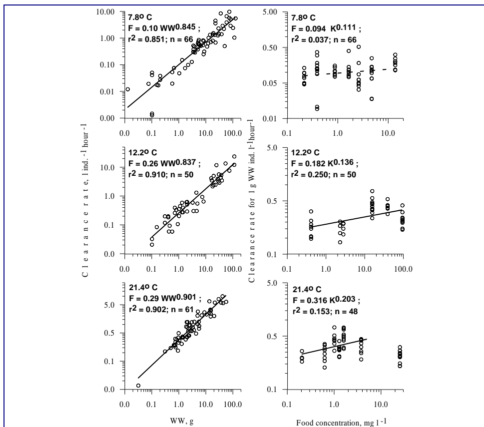
Figure 3.6. Relationships between individual wet weight (WW, g) and temperature dependent clearance rate (l ind. -1 hour -1 ) (left blocks) and between temperature dependent clearance rate of 1g WW individual (l ind. -1 hour -1 ) and food concentration (mg l -1 ) (right blocks) of the jellyfish Aurelia aurita from the Black Sea
