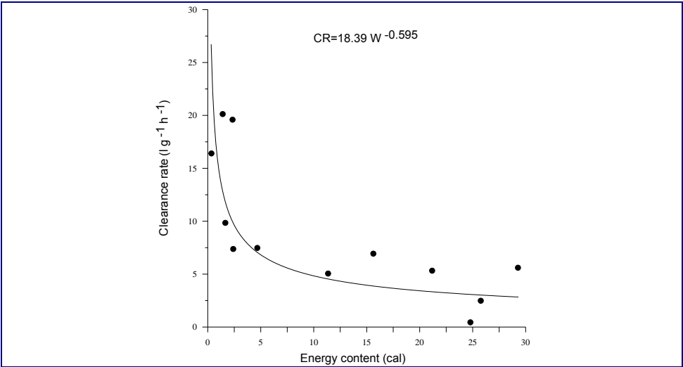
Figure 4.4. Relationship between specific clearance rate ( \text{l g}^{-1} \text{DW h}^{-1} ) and body energy content ( \text{cal ind.}^{-1} ) in M. leidyi
