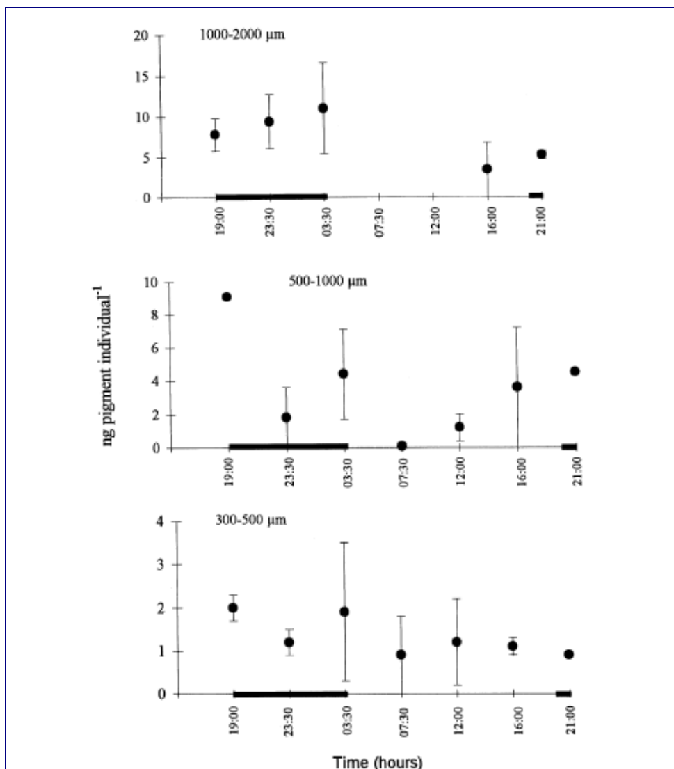
Figure 1.5. Diel gut fluorescence for three size fractions of copepods sampled from 50 m to the surface in September 1995. Each point represents mean \pm SD. Shaded bar along the x-axis indicates the dark hours.
