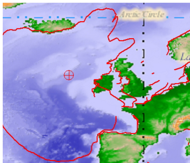
Fig. 5. Preliminary Joint Research Centre model output for tsunami propagation around the coasts of Europe from a source in the North Atlantic. Red lines indicate tsunami travel time in 2 h intervals.
