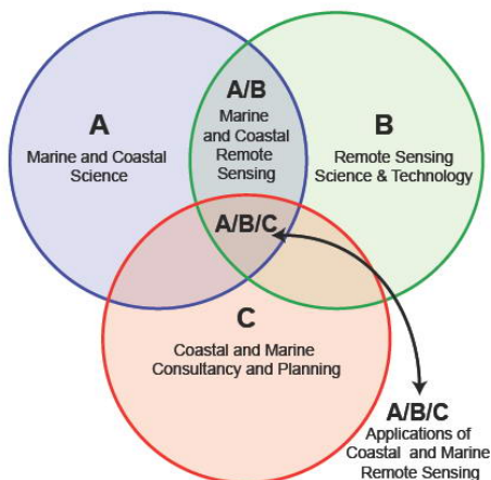
Figure 1. Professional domains contributing to coastal and marine remote sensing. Modified from Robinson, 1988.
