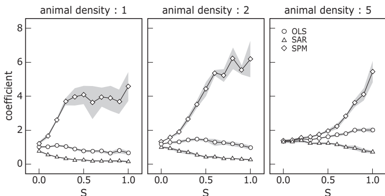
Figure 3.3. Estimated direct and total food effects for an intermediate level of interference ( q = 0.5 ), intermediate smoothness ( r = 3 ), conspecific attraction ( s ) as indicated in each panel, animal densities 1, 2, 5 and \theta = 0 . The 95% confidence intervals are indicated by bands. Confidence intervals for \beta_{1SAR} and \beta_{1OLS} are very narrow and therefore do not come through everywhere. OLS = Ordinary Least Squares model; SAR = Spatial Autoregressive model; SPM = Total average food effect based on the SAR regression coefficients and the spatial multiplier. Similar results hold for other values of q and r .
