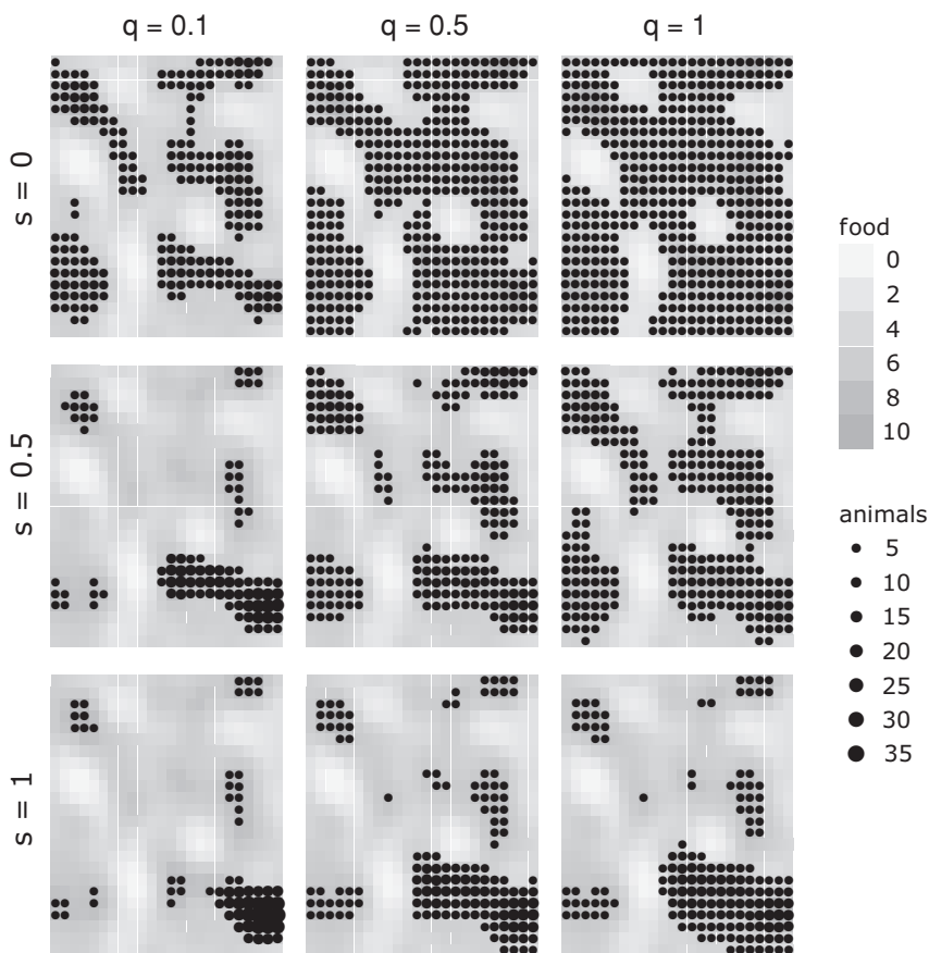
Figure 3.1. Spatial distribution of omniscient animals ( \theta = 0 ) in a fixed and smoothed ( r = 5 ) 24 \times 24 cells resource landscape with mean animal density equal to 1 individual per cell. Each panel is based on one simulation run for a given combination of s (conspecific attraction parameter) and q (interference parameter). Colour intensity of the landscape represents food density and the size of the dots represent the number of animals.
