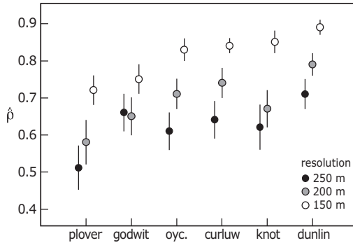
Figure 4.2. Spatial dependence ( \hat{\rho} ) by resolution and shorebird species in the Dutch Wadden Sea.
