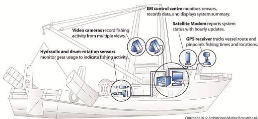
Figure 5.4. Schematic of an electronic monitoring system illustrates the main components and typical placement on a fishing vessel.
