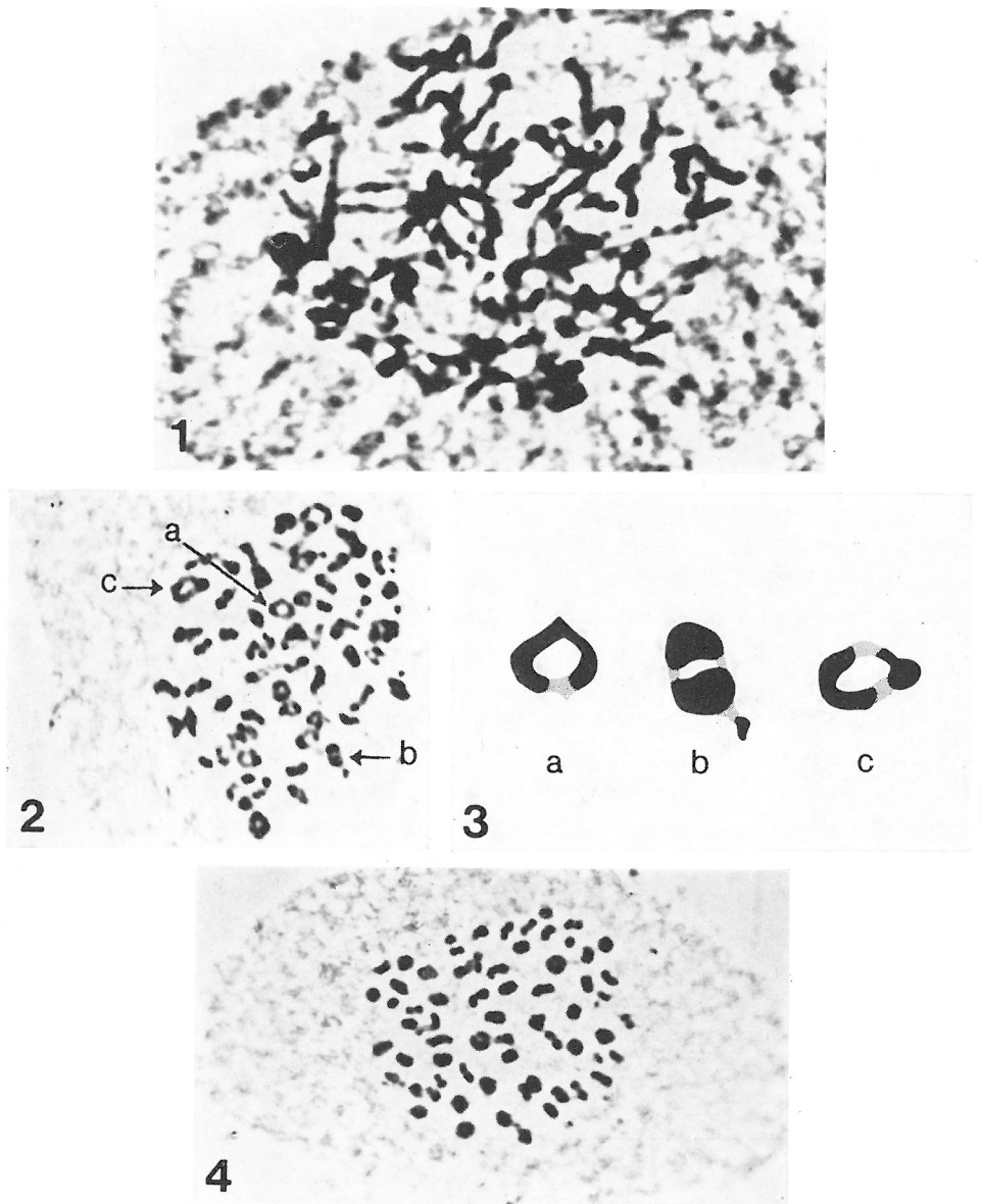
Fig. 1. — Pachytene division from H. americanus testis.
