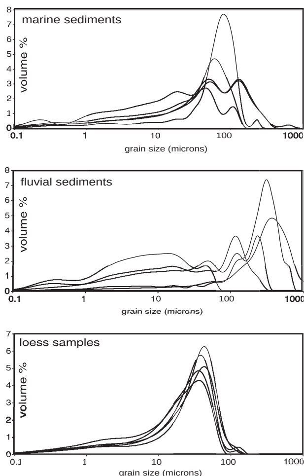
Figure 1. Examples of laser-diffraction grain-size distribution curves of marine, fluvial, and loess samples. For clarity, all distributions have been cut off at 0.1 and 1000\text{ }\mu\text{m} (the measurement range was 0.04\text{--}2000\text{ }\mu\text{m} ).
