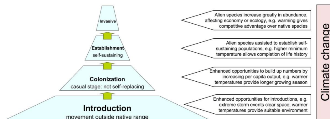
Figure 1. Stages in the sequential transitions of a successful invasion process, modified from Walther et al. 's (2009) figure 1 and associated text.
