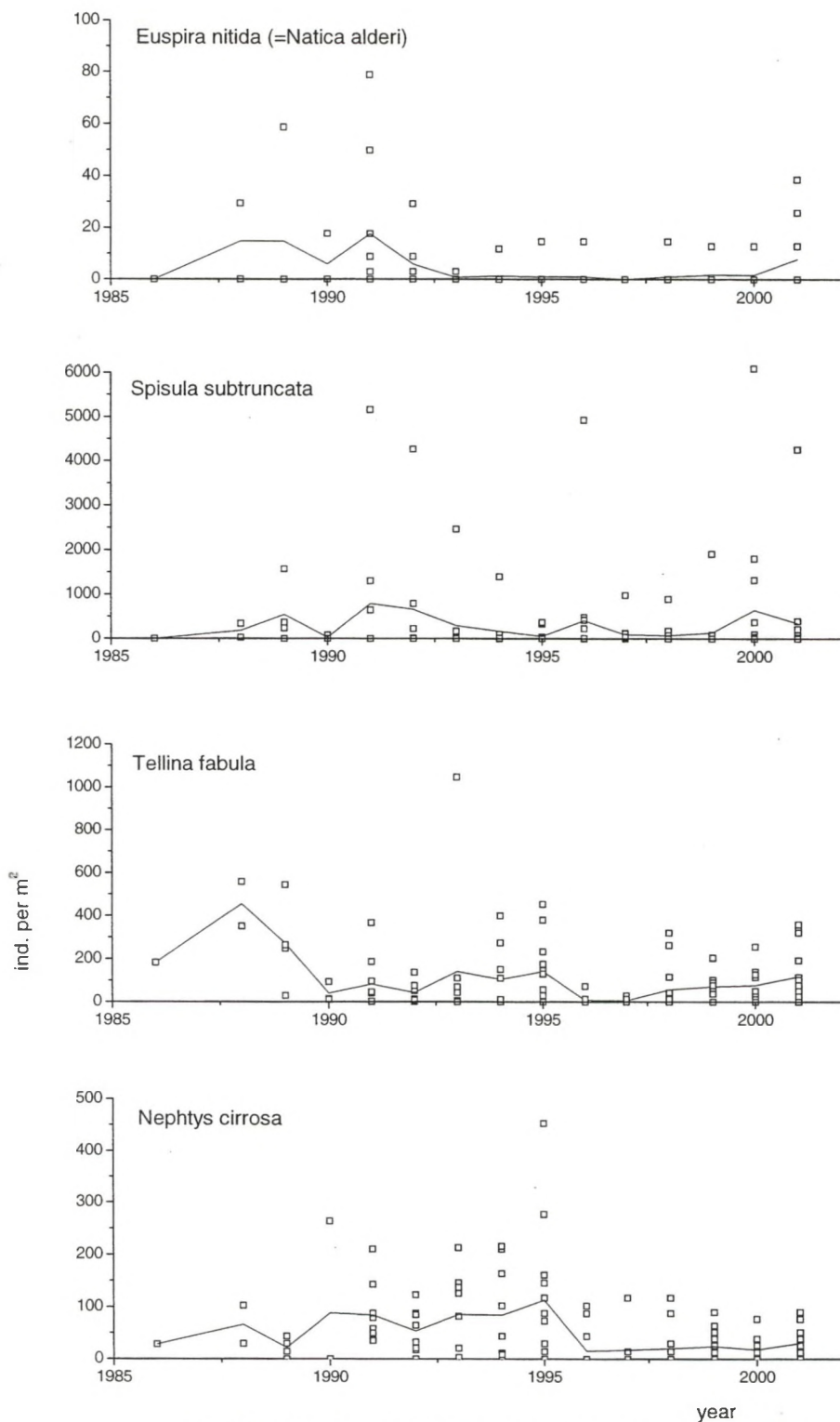
Fig. 16b: Densities of 4 species in the coastal area (1986-2001)
