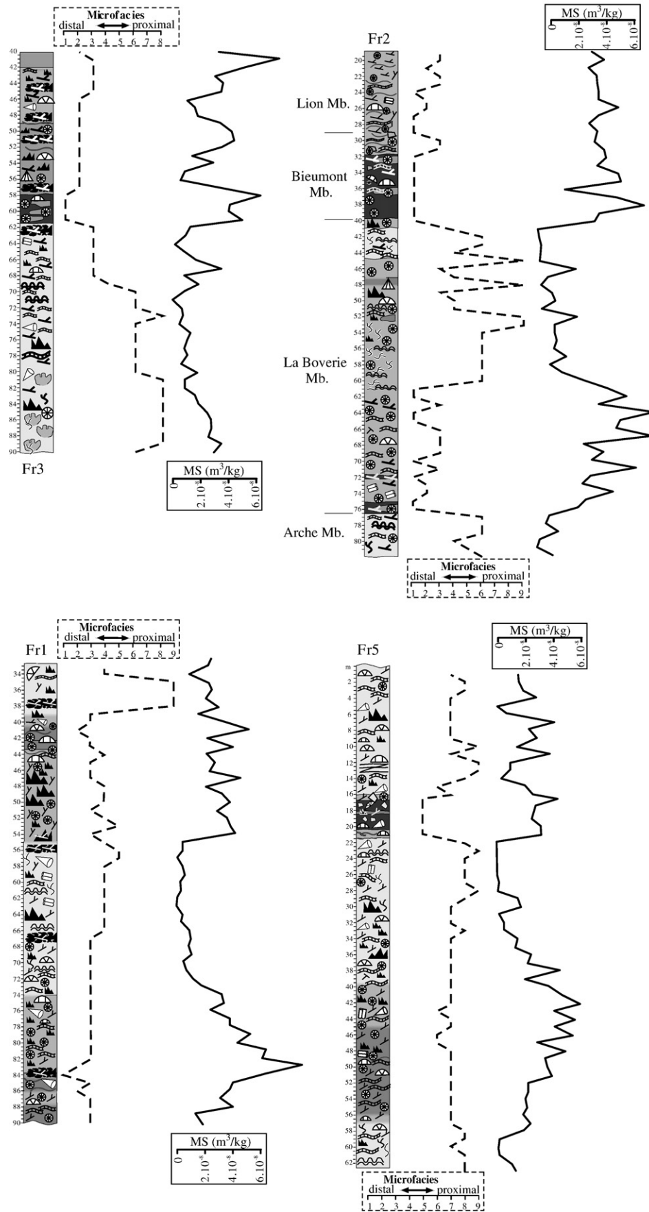
Fig. 9. Lithologic successions of the boreholes drilled in the Nord quarry at Frasnés with facies evolution (dotted lines, Belgian mound and atoll facies model, BMA) and magnetic susceptibility curves (MS). This figure shows that for the carbonate mound MS decreases toward the shallowest microfacies. Legend is in Fig. 7F.
