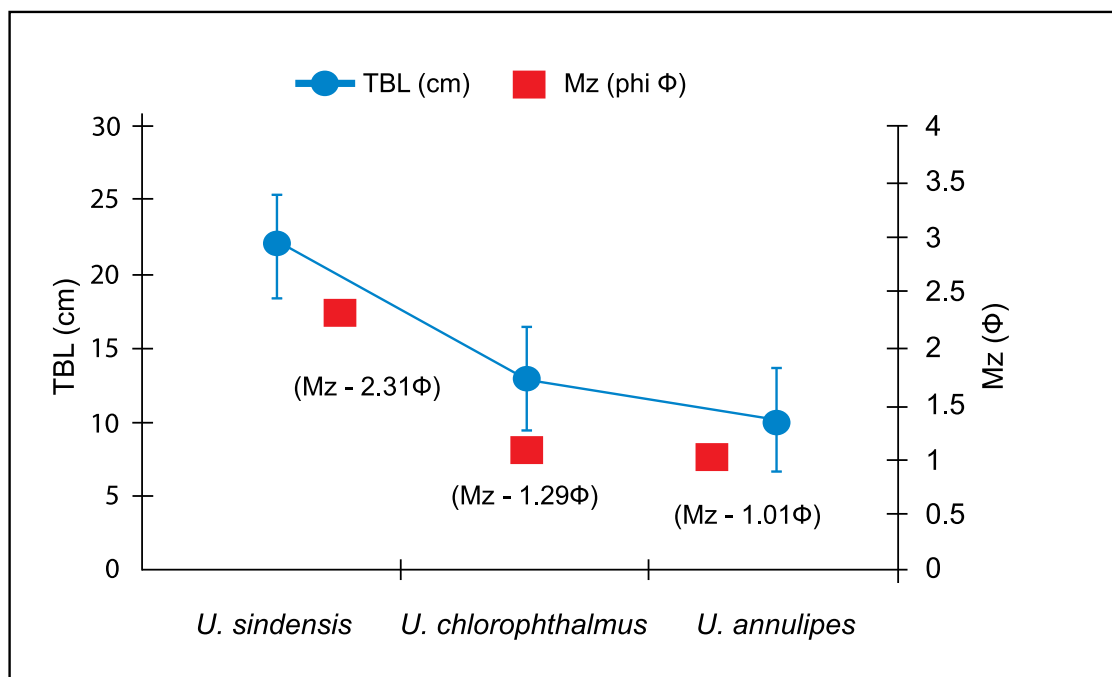
Fig. 3. – The average total burrow length (TBL) of three species of fiddler crab ( Uca sindensis , U. chlorophthalmus , U. annulipes ) in relation to mean sediment (Φ) grain size.
