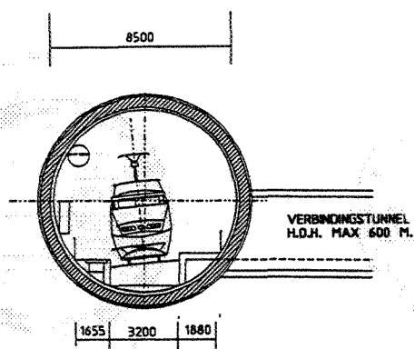
5. TREIN 250 KM/H, ENKEL SPOOR
