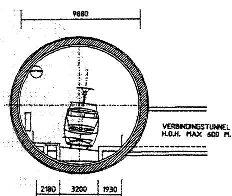
8. TREIN 300 KM/H, ENKEL SPOOR
