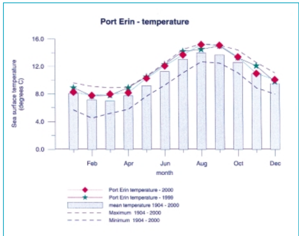
Surface seawater temperature at Port Erin. Monthly means for years 2000 and 1999, with long-term minima, maxima and monthly means 1904 to 2000.
