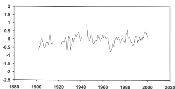
Filtered temperature anomaly
