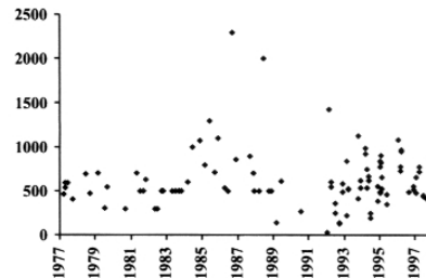
Total Oxidised Nitrogen
