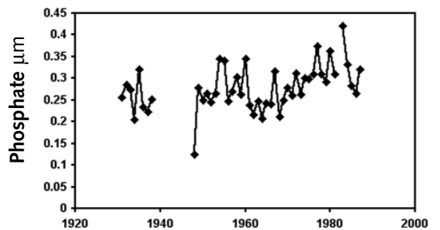
Silicate and Phosphate concentrations at Station E1, off Plymouth
