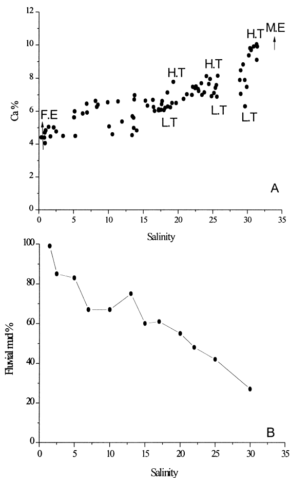
Fig. 4. (A) Calcium content in the SPM at the six stations. Samples collected at high tide (H.T) and low tide (L.T), the marine end member (M.E) and the fluvial end-member (F.E), indicated by the arrow are highlighted in the figure. (B) The percentage of fluvial material calculated with the Ca content in the SPM is presented as function of salinity.
