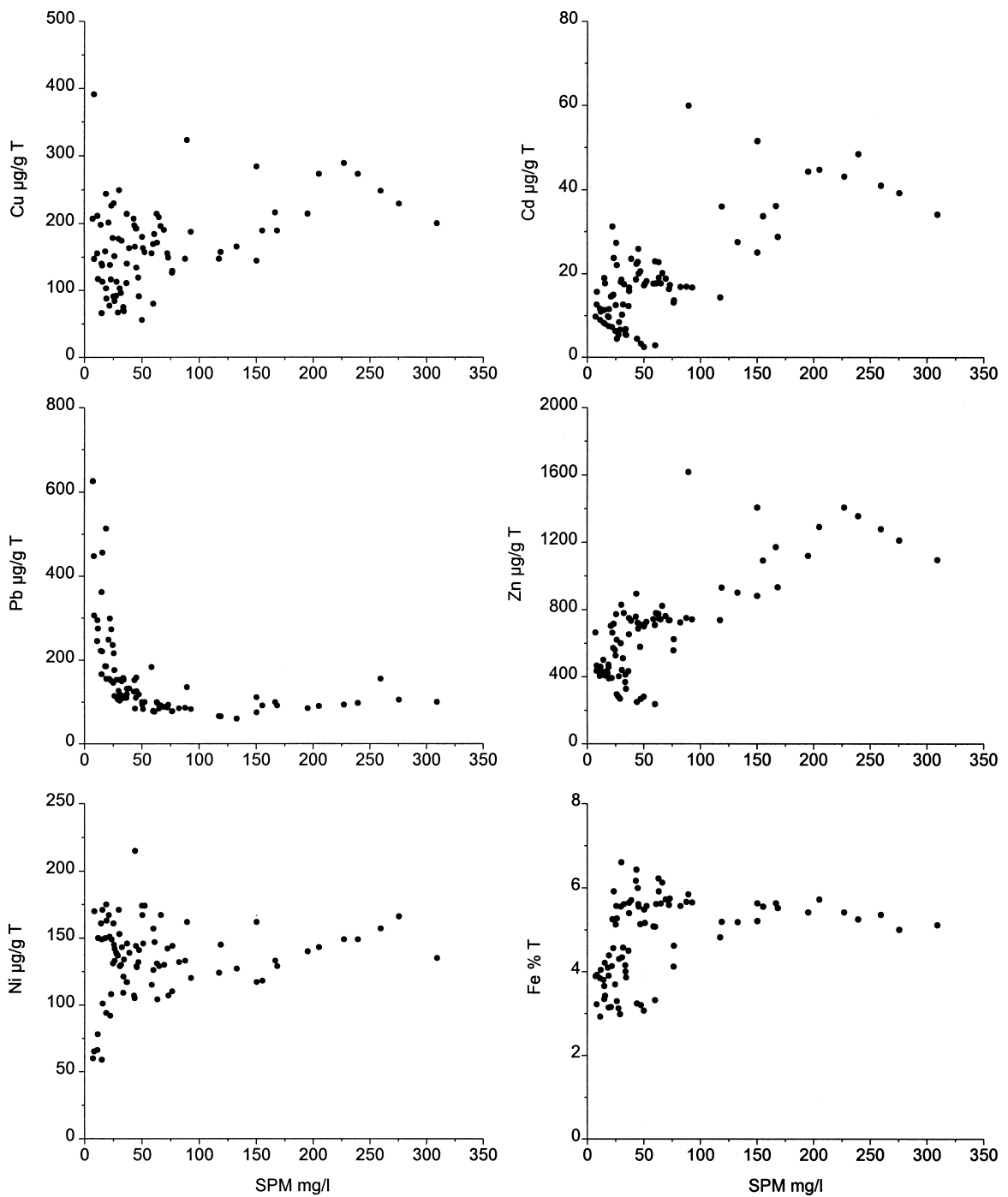
Fig. 11. Total concentrations of particulate Cu, Cd, Pb, Zn, Ni ( \mu\text{g g}^{-1} ) and Fe (%) as function of the amount of suspended matter ( \text{mg dm}^{-3} ).
