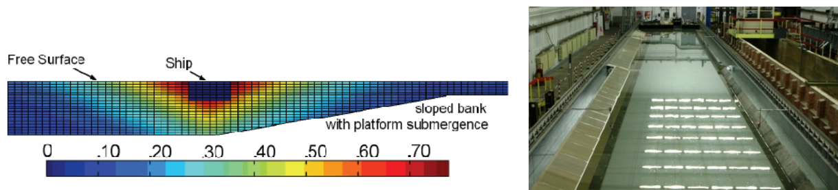
Figure 7: Graphical presentation of weight distribution (left) and four bank types in the towing tank (vertical wall, slope 1/1, 1/3 and 1/4)
