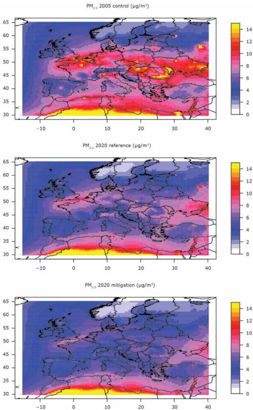
Figure 5.5 Annual average maps of PM_{2.5} ( \mu g/m^3 ) modelled with Chimere: 2005 control, 2020 reference and 2020 mitigation
