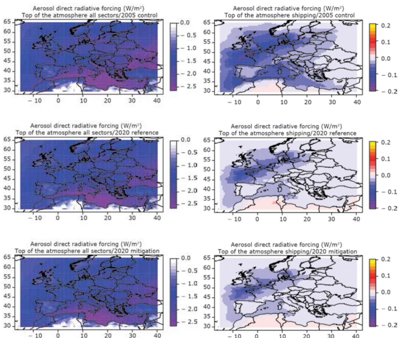
Figure 6.2 Left: aerosol-induced direct radiative forcing (in \text{W/m}^2 ) at the top of the atmosphere in the control (2005) and the two projections: reference (2020) and mitigation (2020); right: the contribution ( \text{W/m}^2 ) attributed to shipping activities
