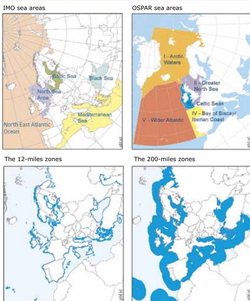
Figure 4.2 Boundaries of international sea areas around Europe
