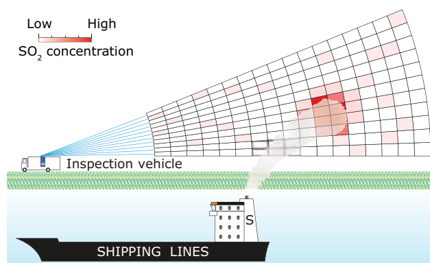
Figure 3.3 Side view of the situation during a \text{SO}_2 emissions measurement by LIDAR
