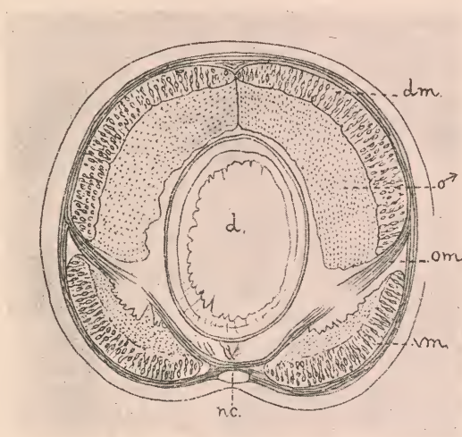
FIG. 147.—Transverse section of the posterior region of a male Polymnia nebulosa .
