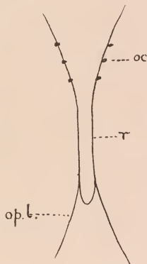
FIG. 140.—Sketch of the folds and eye-spots of a young example of Sabellaria alveolata . oc. , eye-spots; r. , ridge; op.l. , opercular lobes. After an outline by Arnold Watson.
