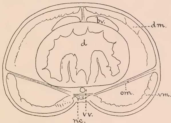
FIG. 146.—Transverse section of the anterior region of Polymnia nebulosa , Mont. Enlarged. bv. , branchial vessels; other letters as before.
