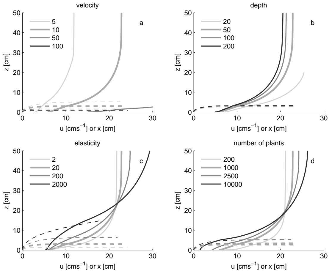
Fig. B-5.2: Flow velocity profiles (continuous lines) and plant positions (dashed lines) in a flume for a) various depth-averaged velocities ( \text{cm.s}^{-1} ); b) various flow depths (cm); c) various elasticities (MPa); d) different plant densities ( \text{per m}^2 ).
