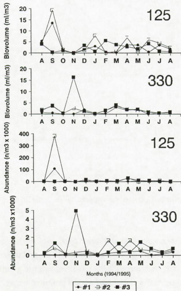
Figure 5 - Zooplankton biovolumes and densities over the annual cycle, for both nets used (125 and 330 \mu\text{m} of pore aperture).
