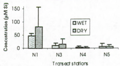
Fig. 5b: NYALI WATER COLUMN: Silicates seasons and variations (1997-98)
