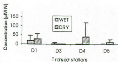
Fig. 2a DIANI WATER COLUMN: Nitrate+Nitrite seasons and variations (1997-98)
