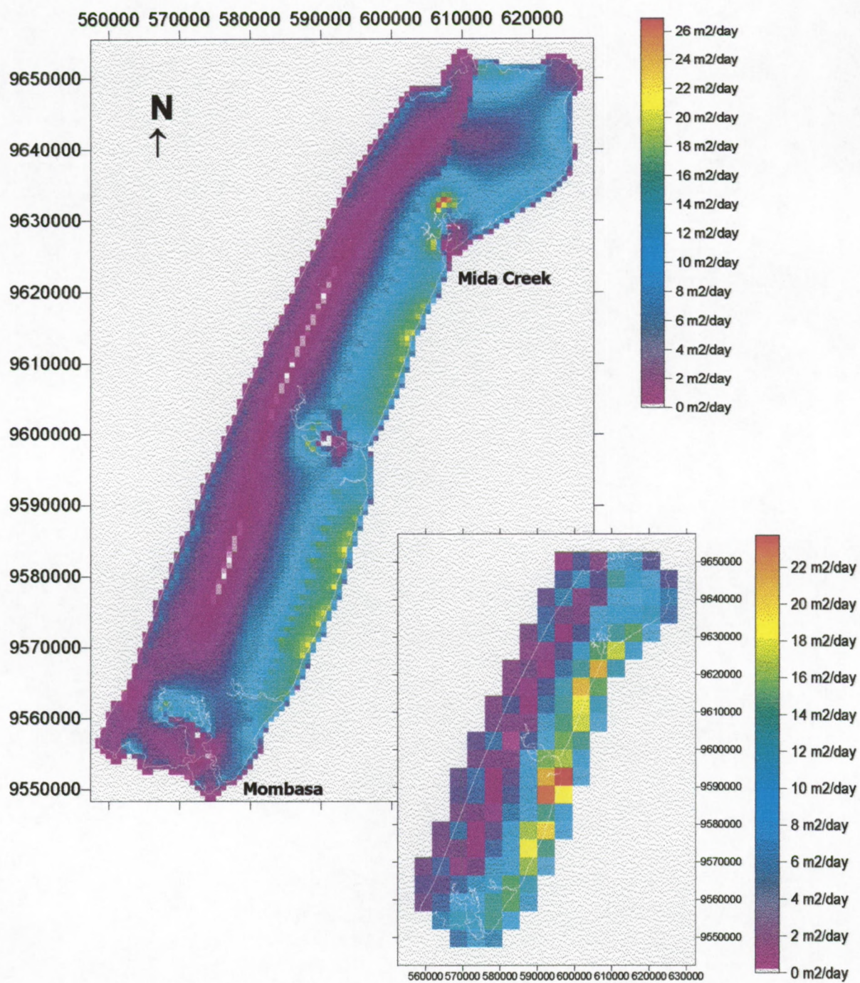
Figure 3: Kenya: groundwater flow velocities ( \text{m}^2.\text{day}^{-1} ) in the area between Malindi and Mombasa (grid sizes: 150x250 m and 5x5 km).
