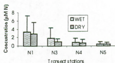
Fig. 3b: NYALI WATER COLUMN: Ammonium seasons and variations (1997-98)
