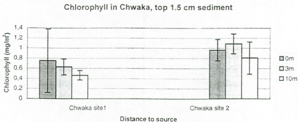
Fig 6. Mean chlorophyll a levels in surface sediments taken at different distances from groundwater outlet points in Chwaka Bay. Values are in mg Chl a.m -2 with standard deviation bars.
