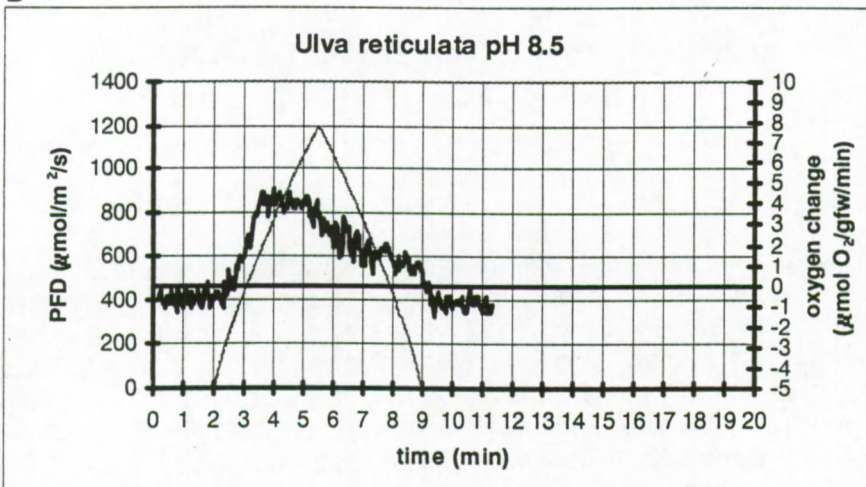
Figure 5 Typical dose response curves for photosynthetic oxygen evolution in macrophytes. Shown here are the effect of pH on the light saturation values and photosynthetic rate at light saturation value.
