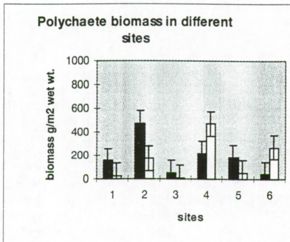
Figure 6: Polychaeta biomass in the different sites for the representative dry season (February 1998, filled bars) and wet season (May 1998, open bars). Numbers on the x-axis refers to the different sites as follows: 1= Paje freshwater site (Pf), 2= Paje normal saline site (Ps), 3=Chwaka freshwater site (Cf), 4= Chwaka normal saline site (Cs), 5= Fumba freshwater site (Ff), 6= Fumba normal saline site (Fs), 7= Makoba freshwater site (Mf), and 8=Makoba normal saline site (Ms).
