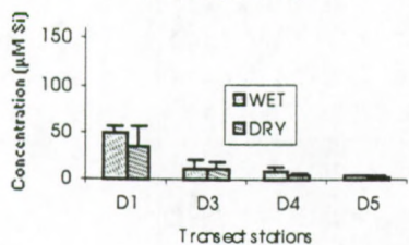
Fig. 5a DIANI WATER COLUMN: Silicates seasons and variations (1997-98)
