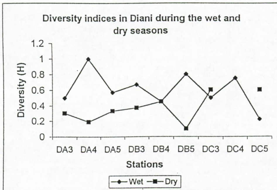
Fig.4. Phytoplankton species diversity during the dry and wet season in Nyali and Diani lagoons.
