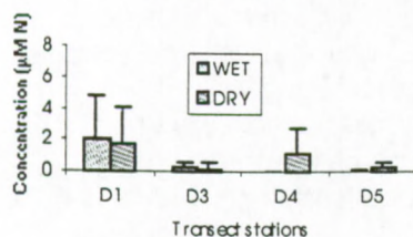
Fig. 3a DIANI WATER COLUMN: Ammonium seasons and variations (1997-98)
