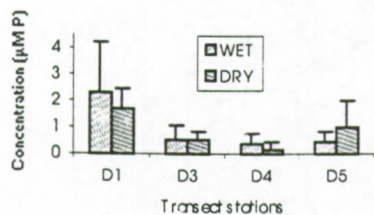
Fig. 4a DIANI WATER COLUMN: Phosphates seasons and variations (1997-98)
