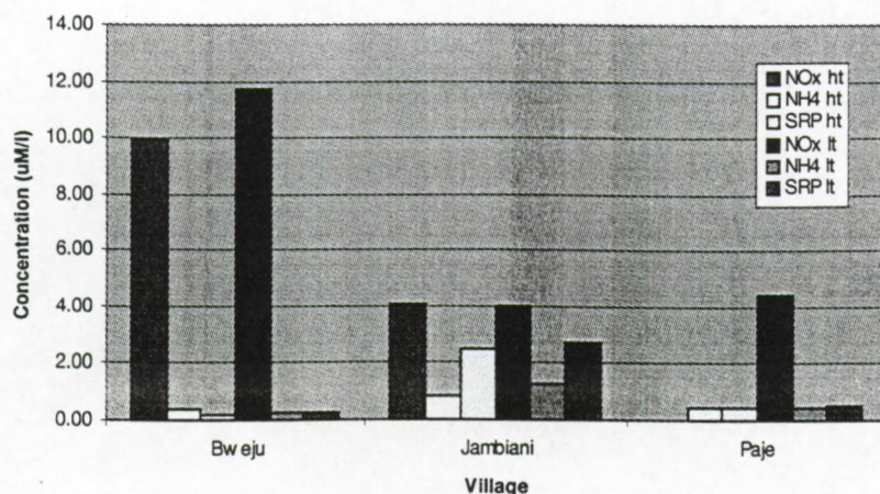
Fig 2 Graph of mean nutrient concentrations at high (ht) and low tide (lt) for each of the villages showing clear tidal influence.
