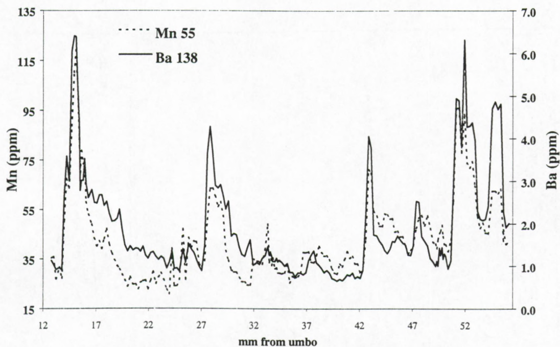
Fig. 7. Mg, Sr, Ba and Mn distribution in the calcitic layer of Isognomon shell T1 from Tudor, analysed by LA-ICP-MS along maximum growth axis
