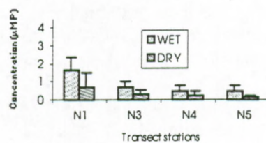
Fig. 4b: NYALI WATER COLUMN: Phosphates seasons and variations (1997-98)
