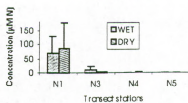
Fig. 2b: NYALI WATER COLUMN: Nitrates+Nitrites seasons and variations (1997-98)
