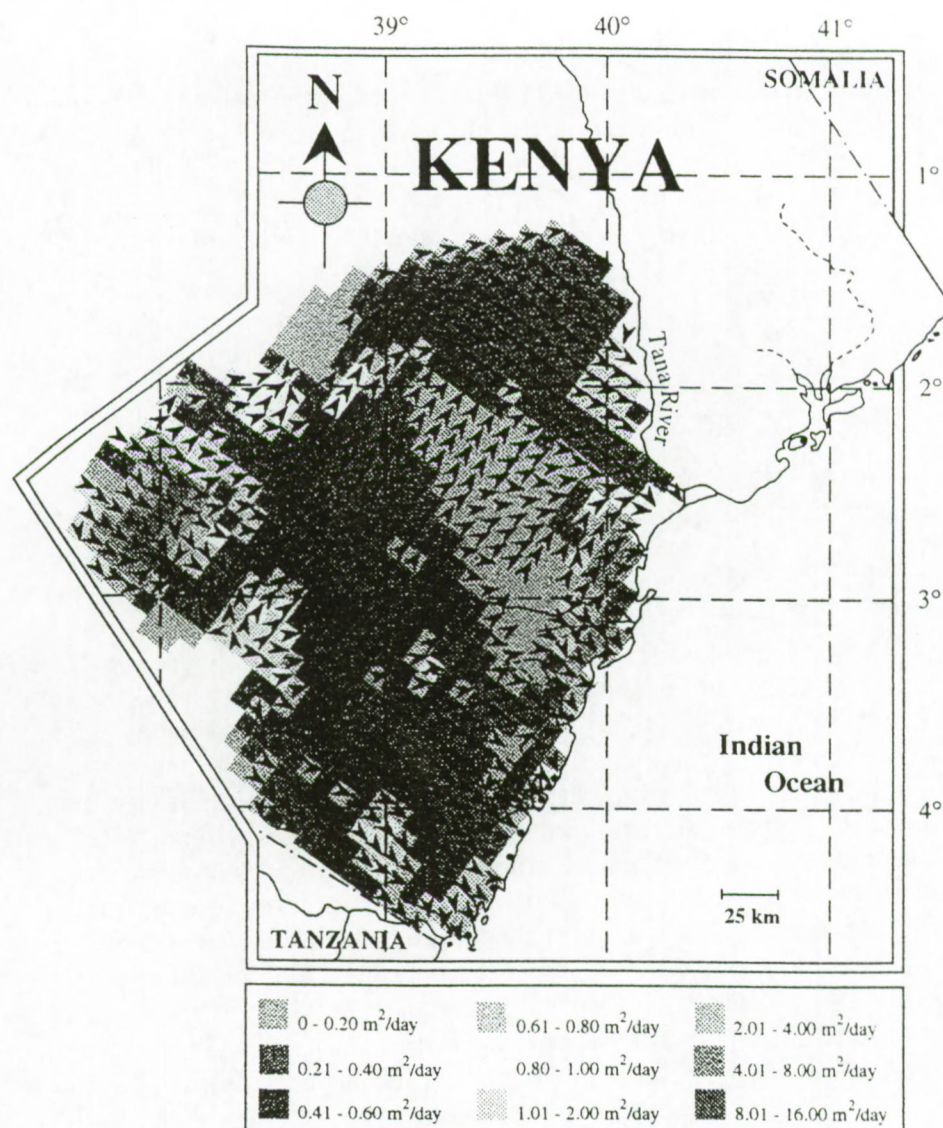
Figure 6. Groundwater flow: graphical output of the model. Arrowheads show the direction of the groundwater flow. Background colours indicate the size of the groundwater flow ( \text{m}^2/\text{day} ).
