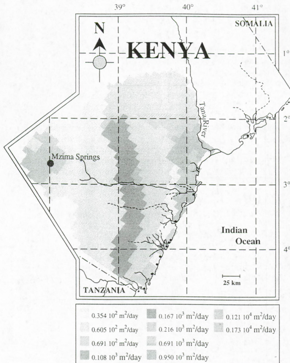
Figure 3. Zones with equal mean transmissivity (m 2 /day) in the study area (Kenya).
