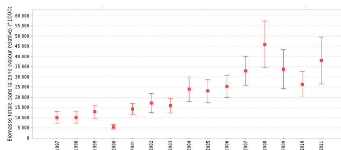
Figure 5.4.41.2 Lesser-spotted dogfish in the Celtic seas. Temporal trends in relative biomass in the French Divisions VII-f-j EVHOE-WIBTS-Q4 survey.
