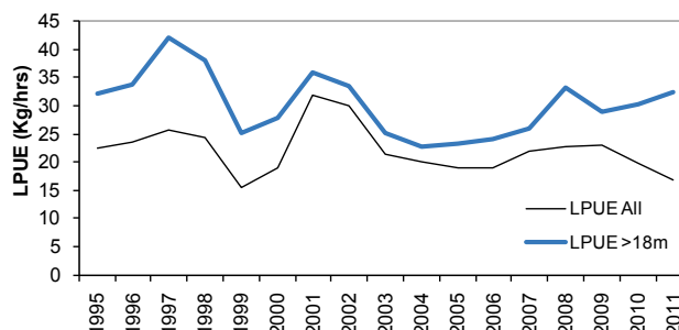
Figure 5.4.34.5.1 Nephrops off the southeastern and southwestern coasts of Ireland (FU 19). Left: Long-term trends in landings (tonnes). Right: Landings per unit effort (lpue, \text{kg hr}^{-1} ) for all vessels targeting Nephrops (black line) and for vessels >18 m total length (blue line).
