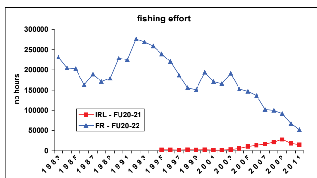
Figure 5.4.34.6.2 Nephrops in the Celtic Sea (FUs 20–22) and in the Labadie area (FUs 20–21). Fishing effort by country (the threshold of Nephrops by weight in total landings is 10% for the French and 30% for the Irish tuning fleets). French indices include FU 22. The French fleet has taken almost 90% of the landings in FUs 20–21 since 1999).
