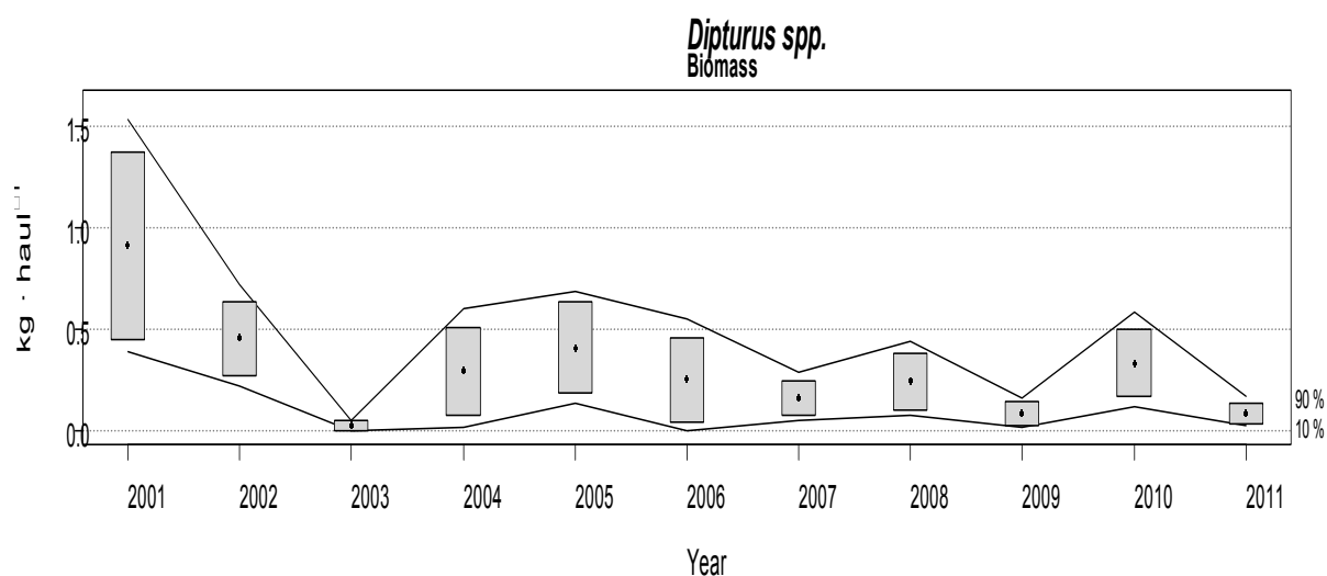
Figure 5.4.42.15.3 The common skate ( Dipturus batis ) complex in the Celtic Sea ecoregion. Temporal changes in the common skate complex biomass ( \text{kg haul}^{-1} ) during the Porcupine survey time-series (2001–2011). Boxes mark parametric standard error of the stratified biomass index. Lines mark bootstrap confidence intervals ( \alpha = 0.80 , bootstrap iterations = 1000). Source: SpPGFS-WIBTS-Q4 survey.
