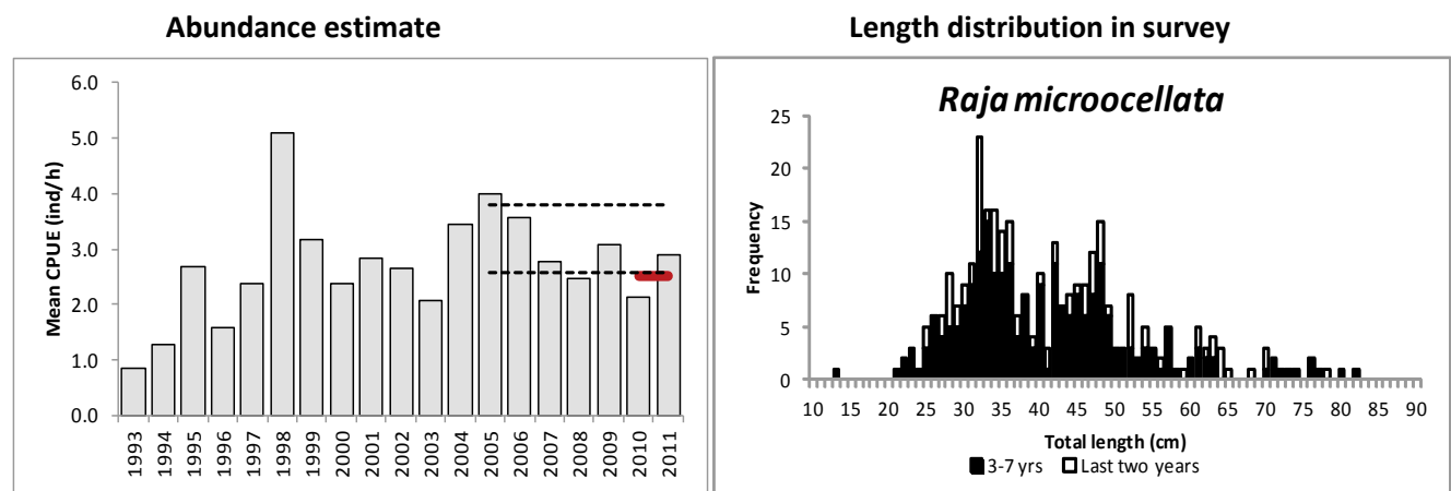
Figure 5.4.42.7.1 Small-eyed ray ( Raja microocellata ) in Divisions VIIIf, g. Left: Mean cpue of Divisions VIIa, f small-eyed ray. Dashed lines indicate the mean annual cpue for 2005–2009 \pm 1 std. dev. The red line shows the mean annual cpue for 2010–2011. Right: Length distribution of small-eyed ray for the periods 2005–2009 (black bars) and 2010–2011 (white bars). Source: UK (E&W) VIIaf BTS survey.
