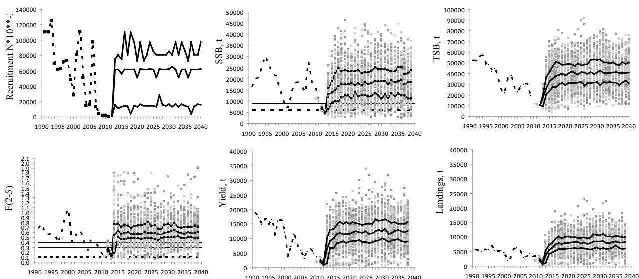
Figure 5.3.3.2 Summary plots of true population values from the 100 simulation iterations for the Excel MSE, assuming medium recruitment, TAC constraint, and discards. The top panels show: recruitment (left), SSB (middle), and total stock biomass (right). The bottom panels show: F (left), yield (i.e. total catch; middle), and landings (right). The solid lines indicate the 25th, 50th, and 75th percentiles. The thin solid horizontal lines show B_{pa} , F_{pa} , and F_{MSY} . The horizontal dashed lines show B_{lim} and F = 0.1 .
