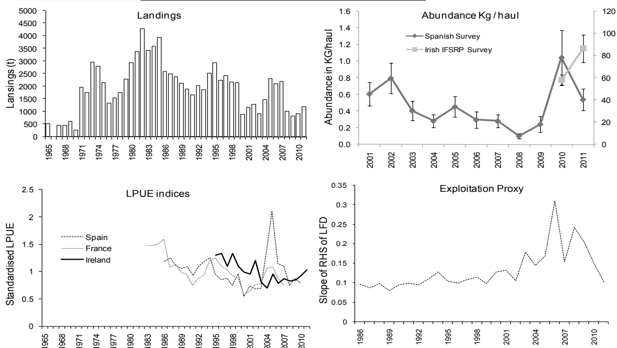
Figure 5.4.34.3.1 Nephrops on the Porcupine Bank (FU 16). Top left: ICES landings. Bottom left: standardized (scaled to mean by index) lpues by fleet. Top right: Abundance estimate (in kg haul -1 ) from Sp-PGFS-WBITS-Q4 and Irish IFSRP surveys. Bottom right: Trends in an exploitation proxy (derived from the slope of the length–frequency for male Nephrops between carapace lengths of 41–56 mm that are considered fully selected in the fishery).
