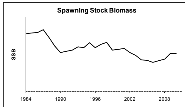
Figure 5.4.19.1 Megrim ( Lepidorhombus whiffiagonis ) in Divisions VIIb–k and VIIa,b,d. Summary of stock assessment (weights in '000 tonnes). Top right: SSB/F for the time series used in the assessment.
