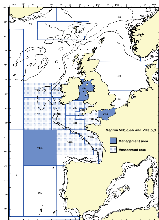
Figure 5.4.19.2 Megrim in Divisions VIIb–k and VIIa,b,d. ICES assessment areas and EU TAC regulation management areas.
