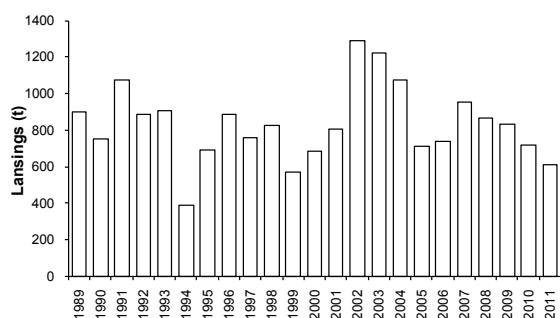
Figure 5.4.34.5.1 Nephrops off the southeastern and southwestern coasts of Ireland (FU 19). Left: Long-term trends in landings (tonnes). Right: Landings per unit effort (lpue, \text{kg hr}^{-1} ) for all vessels targeting Nephrops (black line) and for vessels >18 m total length (blue line).
