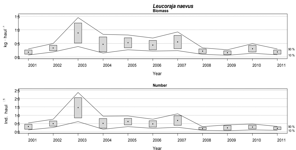
Figure 5.4.42.14.3 Temporal changes in cuckoo ray ( Leucoraja naevus ) biomass index (kg haul -1 )(top) and numbers (numbers per haul) during the Porcupine survey time series (2001–2011). Boxes mark parametric standard error of the stratified biomass index. Lines mark bootstrap confidence intervals ( \alpha = 0.80 , bootstrap iterations = 1000)IGFS trawl survey Q4. Dashed lines indicate the mean \pm 1 std. dev. annual cpue for 2005–2009, the red line shows the mean annual cpue for 2010–2011. Source: SpPGFS-WIBTS-Q4 survey.
