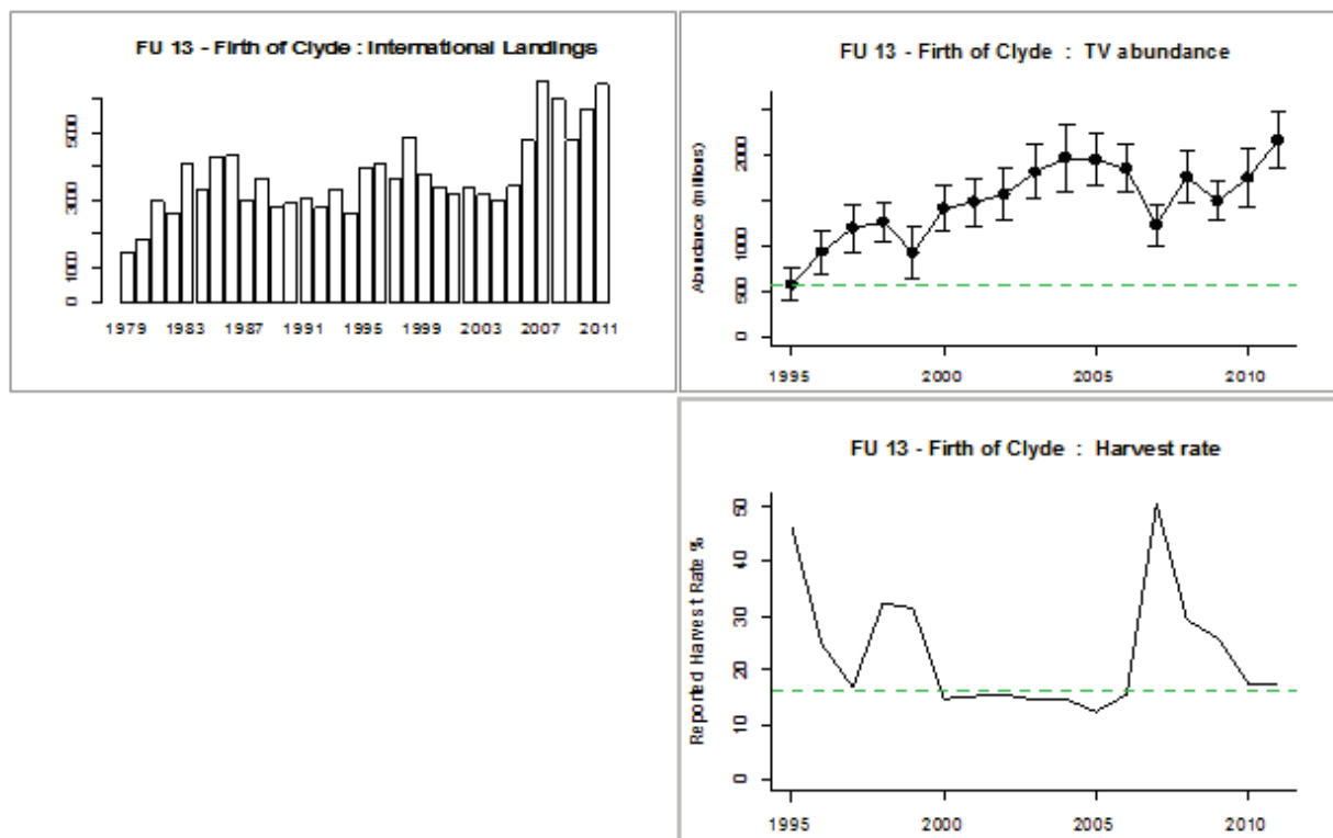
Figure 5.4.33.1 Nephrops in the Firth of Clyde (FU 13). Long-term trends in landings (tonnes), UWTV survey (in millions; SSB proxy), and harvest rate (fishing mortality proxy). Harvest rates before 2006 may be unreliable due to underreporting of landings. Green dashed lines represent MSY B_{trigger} and F_{MSY} harvest ratios.
