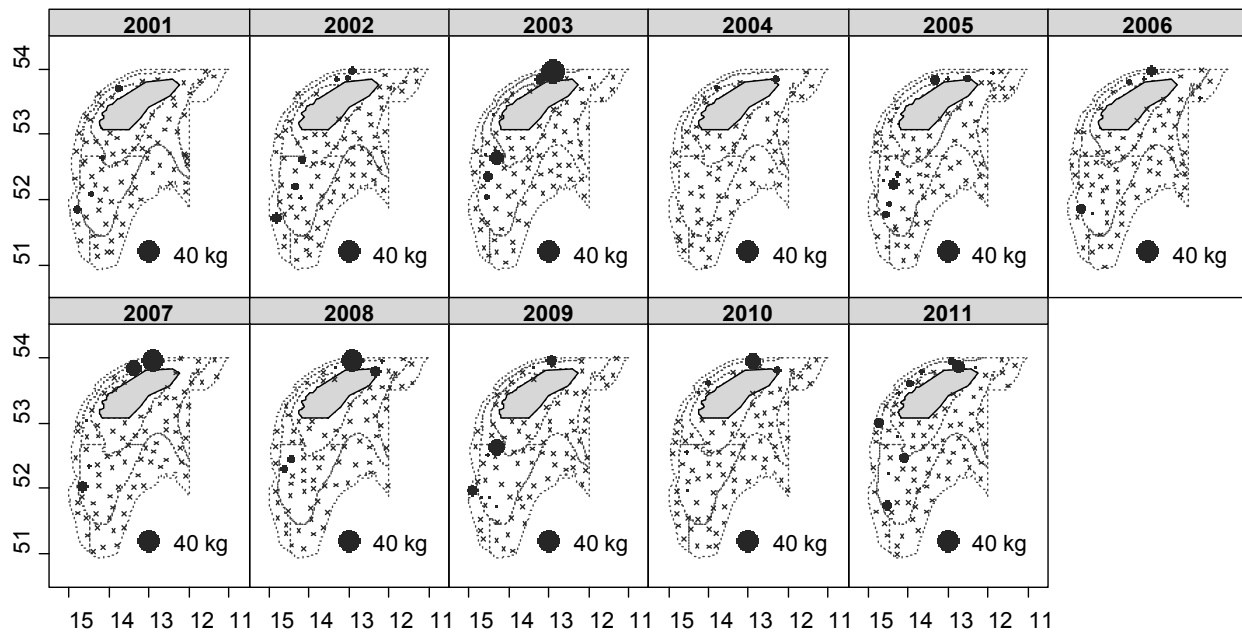
Figure 5.42.12.1 Sandy ray ( Leucoraja circularis ) around the Porcupine bank. Geographical distribution of catches ( \text{kg} \cdot \text{haul}^{-1} ) in the Porcupine survey time-series (2001–2011). Source: SpPGFS-WIBTS-Q4.
