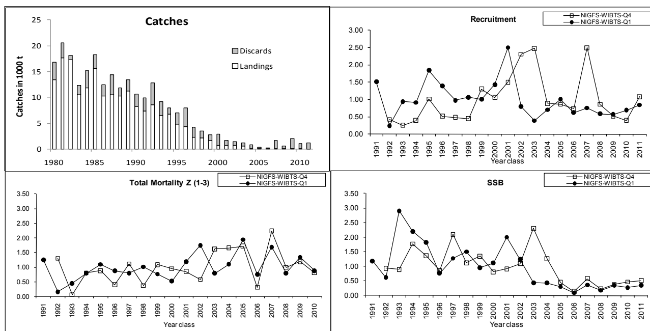
Figure 5.4.5.1 Whiting in Division VIIa (Irish Sea). Catch reported to the WG (in thousand tonnes, 1991–2002 estimates include sampled-based estimates of landings at a number of Irish Sea ports, discards included 1980–2011), and mean standardised: SSB, total mortality (Z), and recruitment estimates, from single fleet SURBA analysis.
