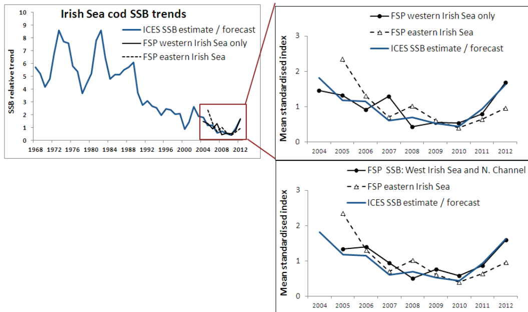
Figure 5.4.1.4 Cod in Division VIIa (Irish Sea). Trends in SSB of cod given by the FSP surveys of the western and eastern Irish Sea and the ICES (2011) assessments. The two right hand plots show the comparisons using the SSB index for the western Irish Sea only (excluding North Channel) and the index including the North Channel (no data for 2004).
