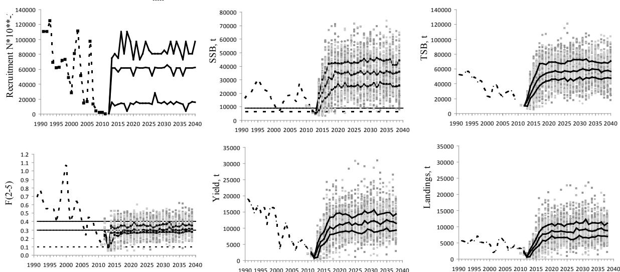
Figure 5.3.3.2 Summary plots of true population values from the 100 simulation iterations for the Excel MSE, assuming medium recruitment, TAC constraint, and discards. The top panels show: recruitment (left), SSB (middle), and total stock biomass (right). The bottom panels show: F (left), yield (i.e. total catch; middle), and landings (right). The solid lines indicate the 25th, 50th, and 75th percentiles. The thin solid horizontal lines show B_{pa} , F_{pa} , and F_{MSY} . The horizontal dashed lines show B_{lim} and F = 0.1 .
