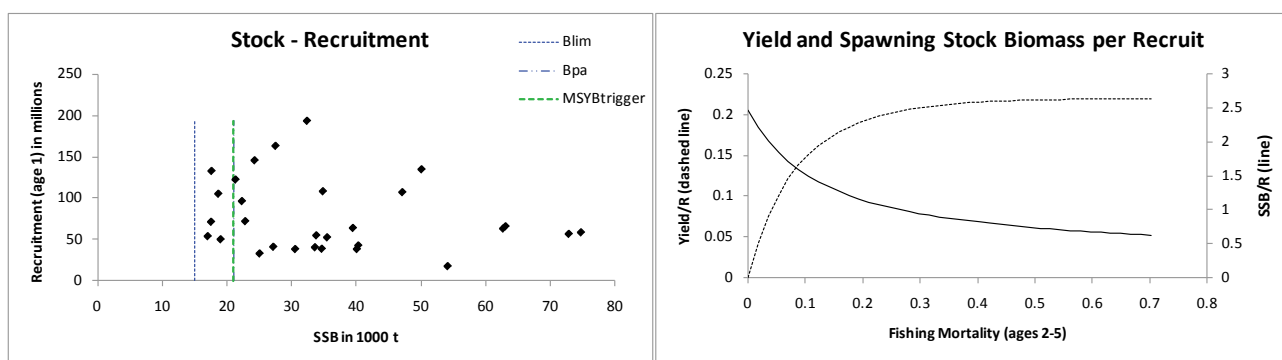
Figure 5.4.6.3 Whiting in Divisions VIIe–k. Stock recruitment plot and yield per recruit analysis..
