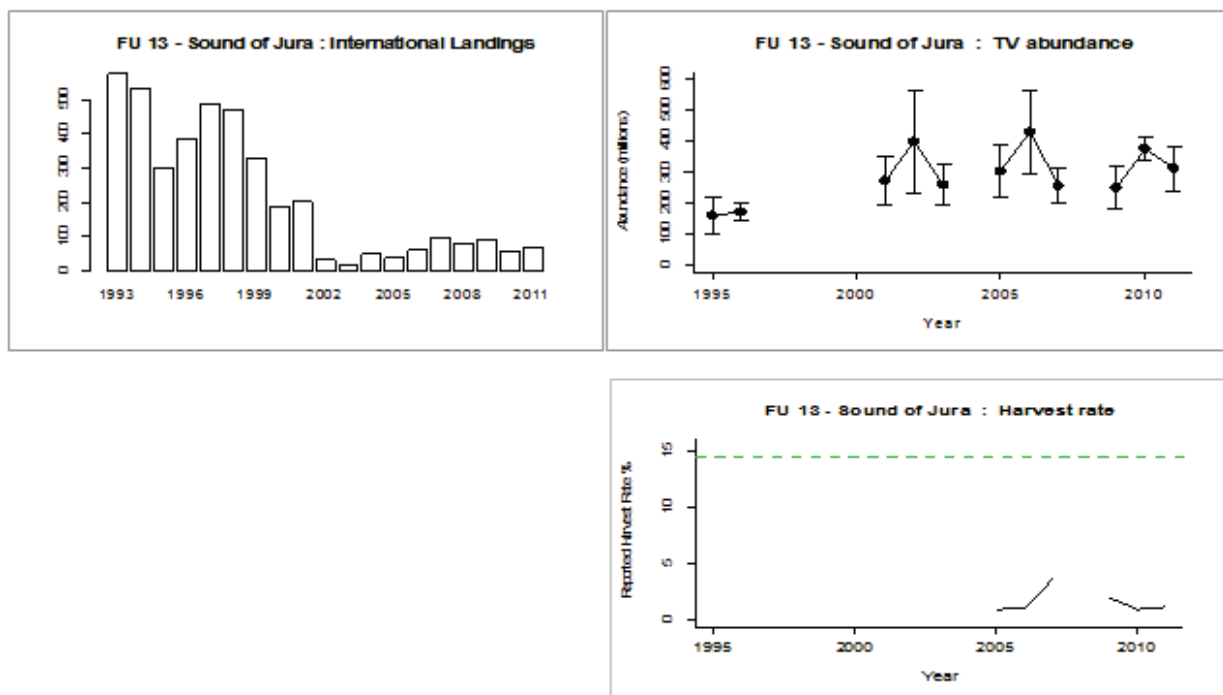
Figure 5.4.33.2 Nephrops in the Sound of Jura (FU 13). Long-term trends in landings (tonnes), UWTV survey (millions; SSB proxy), and harvest rate (fishing mortality proxy, no data available before 2005). Harvest rates before 2006 may be unreliable due to underreporting of landings. Green dashed line represents F_{MSY} harvest ratios.
