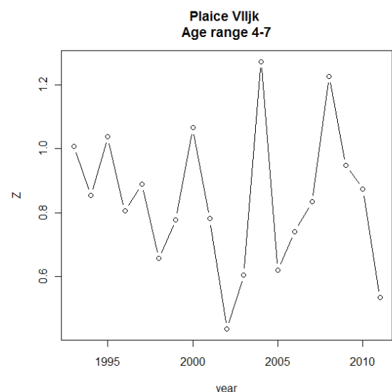
Figure 5.4.10.1 Plaice in Divisions VIIh–k. official landings (left plot). Catch curves analysis (right plot).
