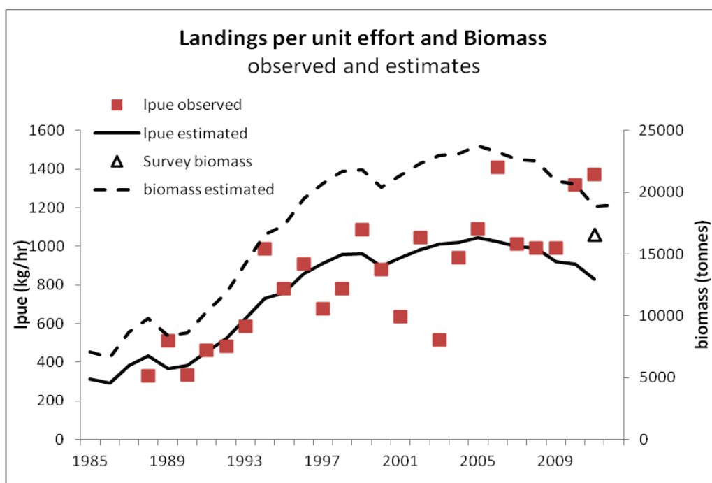
Figure 5.4.18.1 Sprat in Divisions VIIId,e. Surplus production model fit (lines) to the commercial landings per unit effort (lpue) data and the acoustic survey estimate of 16 600 t.
