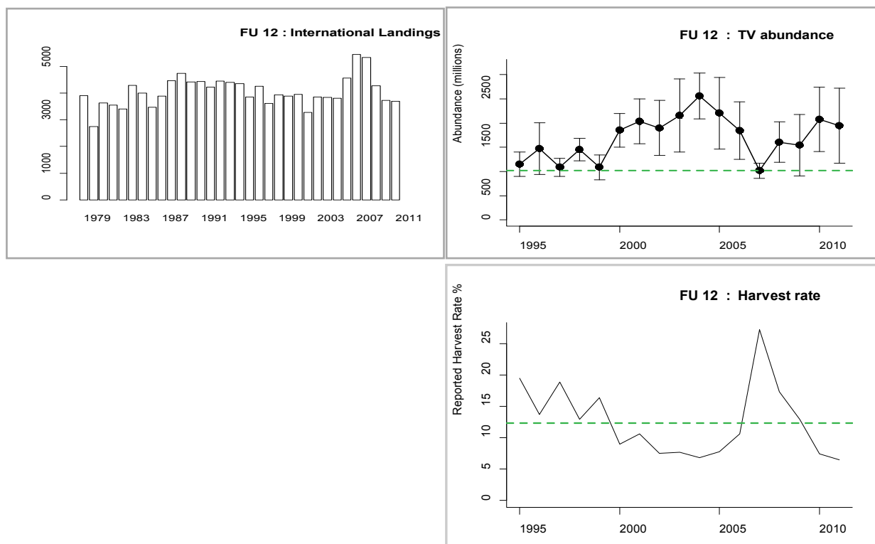
Figure 5.4.33.2.1 Nephrops in South Minch (FU 12). Long-term trends in landings (tonnes), UWTV survey (millions; SSB proxy; Confidence intervals 95%), and harvest rate (fishing mortality proxy). Harvest rates before 2006 may be unreliable due to underreporting of landings. Green dashed lines represent MSY B_{trigger} and F_{MSY} harvest ratios.
