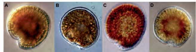
Figure 1. Light micrographs of four newly described Gambierdiscus species, demonstrating their morphological similarities and supporting the need for molecular methods to discriminate species level differences a) G. caribaeus , b) G. carolinianus , c) G. carpenteri , d) G. belizeanus (courtesy of M. Vandersea, NOAA).
