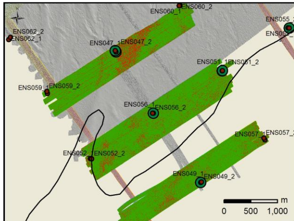
Figure 27. Slope map along northern slope Vlake van de Raan. Areas with rougher seabed correspond to slope values of more than 2° (red). RV Belgica ST1029; data resolution 1x1m.
