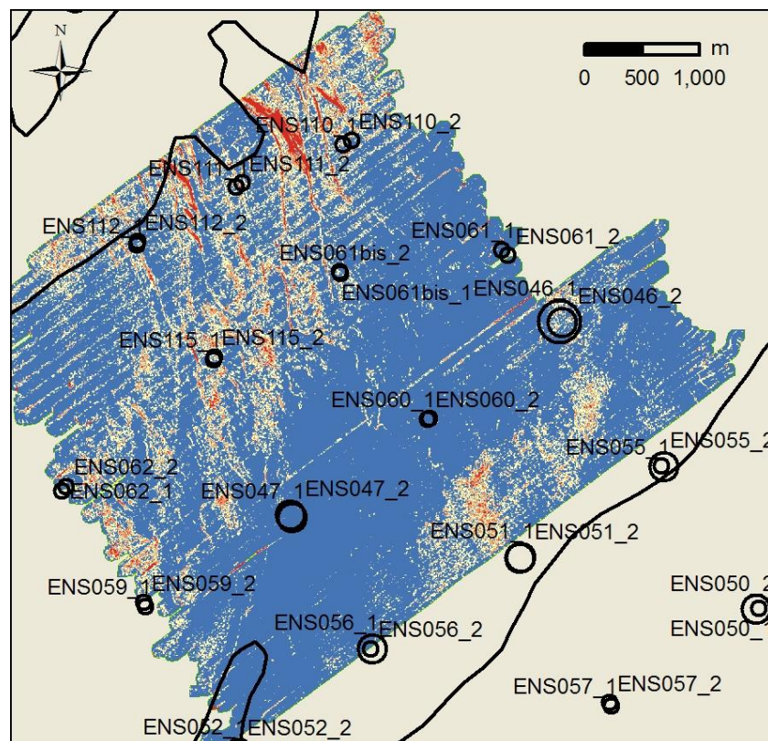
Figure 29. Relative rugosity map (blue to red corresponds to low to high rugosities) along the northern slope of the Vlake van de Raan (Benthic terrain modeller). Higher rugosity values to the north are related to bedforms (see previous figure). It is hypothesized that the higher rugosity to the south (upper slope) are related to higher densities of both E. directus and O. fusiformis . Note the relatively higher rugosity near sampling location 51 (2010), where up to 341 ind/m 2 of E. directus were counted.
