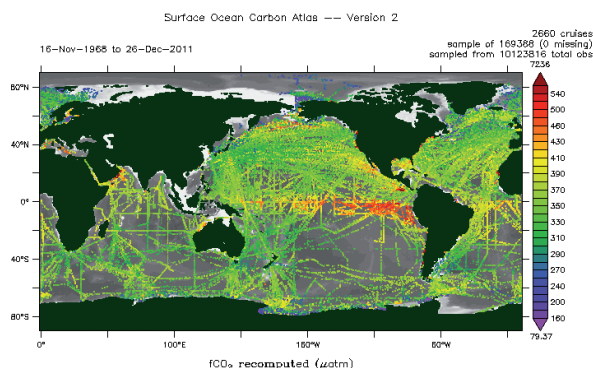
Fig. 1 - Distribution of fCO 2 data using the LAS of SOCAT Version 2.
