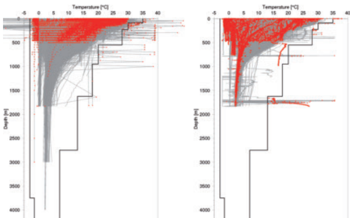
Fig. 2 - Profiles of XBT casts: (left panel) standard depth data, (right panel) high resolution (1m intervals) data. Red circle shows questionable or bad value by range and/or excessive gradient/inversion check and thick line shows temperature acceptable range as a function of depth in the North Pacific Ocean same as WOD09.
