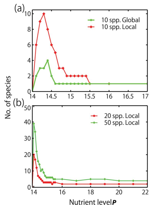
Figure 2 | Species diversity after 20,000 time steps plotted against nutrient level P . (a) The number of surviving species out of ten species under local and global interactions. (b) The number of surviving species out of 20 and 50 species under local interaction.
