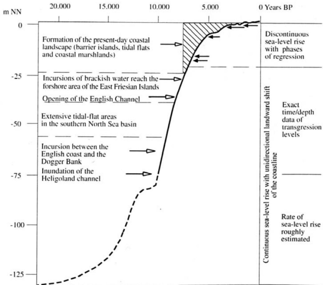
Fig. 2-2: Sea level rise in a time/depth diagram from 20,000 years BP to recent times (Streif 2004)
