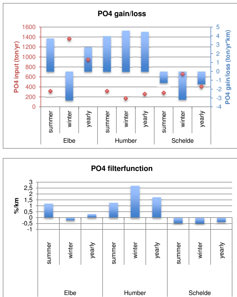
Fig. 38 Sink and source function for phosphate (PO 4 ) in the Elbe, Scheldt and Humber estuary, calculated as six-year average along the whole estuarine gradient on a yearly, summer and winter basis. In the upper graph, input (ton/yr) and gain/loss (ton/yr*km) are given. In the lower graph, contribution of gain/loss relative to the initial input (starting concentration) is displayed (%/km). Summer = June, July, August; winter = December, January and February.
