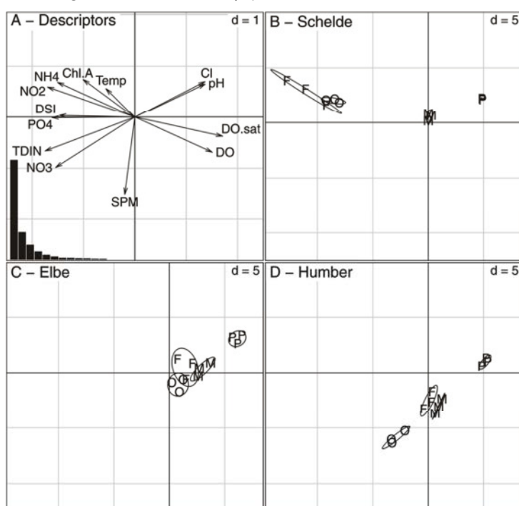
Fig. 24 PTA, Compromise. A) Descriptors and eigenvalues diagram; first axis (horizontal), 79.0 %; second axis (vertical), 11.7 %. B) Statistical units grouped per zone (three years per estuary). “d” indicates the grid scale.
