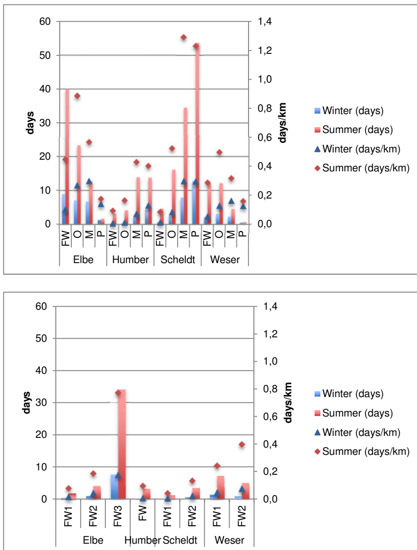
Fig. 10 Winter and summer residence time per zone (days) and normalized for the length of each zone (days/km) of the Elbe, Humber, Scheldt and Weser estuaries calculated according to the fractal freshwater method (Guo et al. 2000, see Vandenbruwaene et al. 2012). The freshwater zone residence times are presented in more detail according to the zonation as decided in (Geerts et al. 2012).
