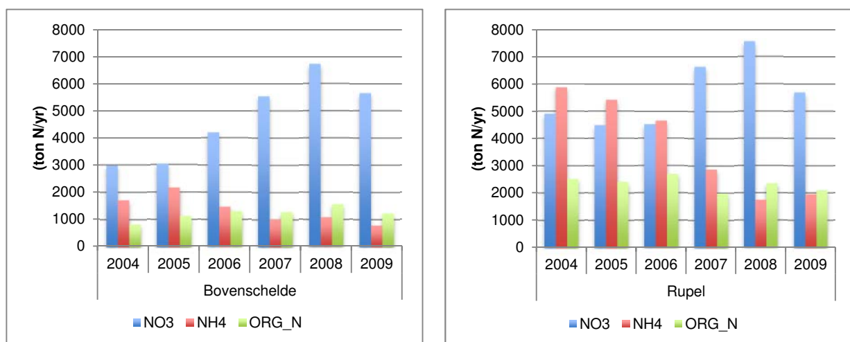
Fig. 48 Yearly changes in nitrogen input in the Scheldt estuary for the most upstream boundary (Bovenshelde) and the main tributary (Rupel) in ton N/yr.
