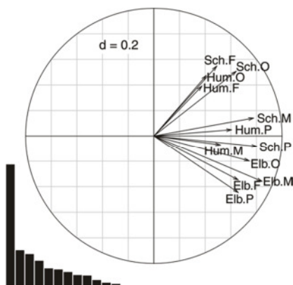
Fig. 19 PTA, Correlation circle of the interstructure. The eigenvalues diagram indicates a highly dominant first value (41,6 %) evidencing common structural similarities among the estuarine zones (contiguous vectors). For labels, see table 4. “d” indicates the grid scale.
