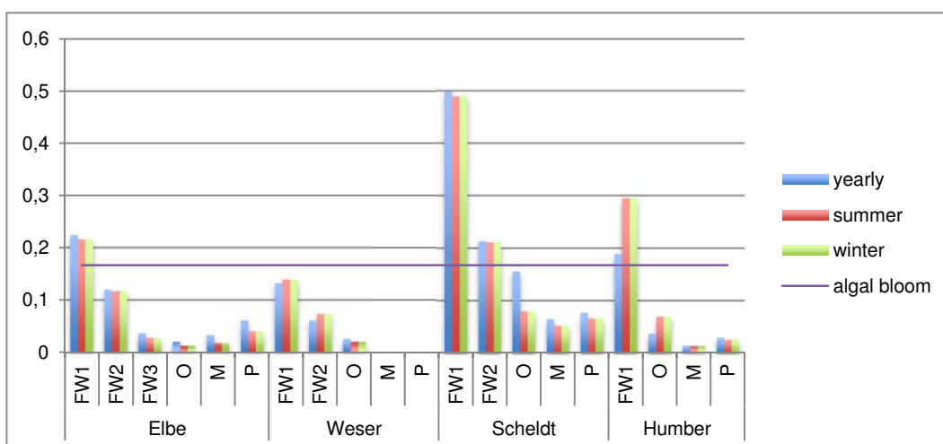
Fig. 16 Six-yearly averaged euphotic depth – mixing depth ratio ( Zeuph/Zmix ) per zone and estuary upon yearly, summer and winter basis. When the Zeuph/Zmix depth is larger than 1/6, algal blooms can occur (Underwood & Kromkamp 1999).
