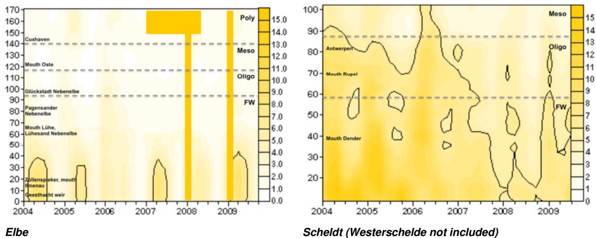
Fig. 47 Spatial (TIDE km) temporal (years) distribution of biological oxygen demand (BOD; mg O 2 /l) for the Elbe and Scheldt. Main tributaries and recognizing sampling points are shown in the surfer plots. Biological oxygen demand is not measured within the Westerschelde and therefore the surfer plot for the Scheldt only goes up to the boundary between the Netherlands and Belgium. Within the Humber and Weser biological oxygen demand is not measured at all and therefore not represented here. The contours displayed here, represent a biological oxygen demand of 5 mg O 2 /l. Missing data in the time-distance plots are represented as solid filled rectangles.
